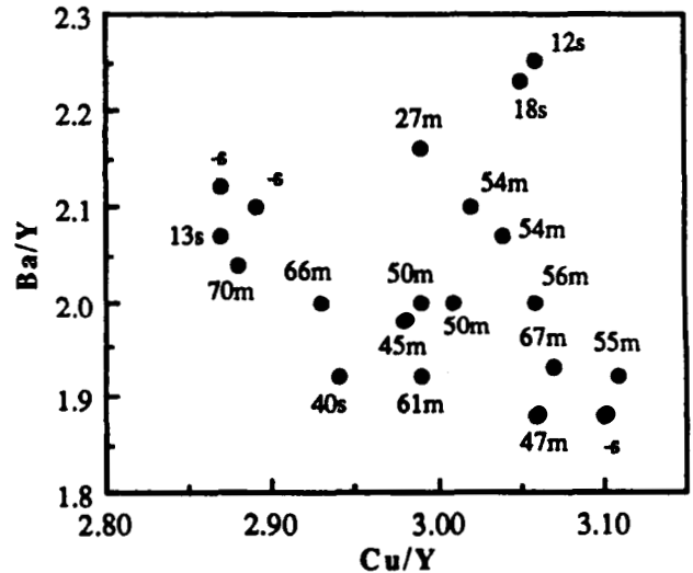
Figure 7: Distribution of T_c for films of various composition on MgO annealed at 850 °C for 3 hr. The number with each point indicates T_c while the letter indicates the behavior in the normal state : metallic or semiconducting.
