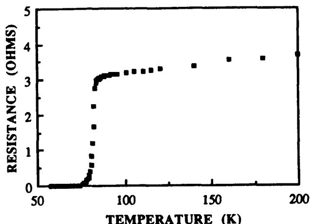
Figure 8: Resistance as a function of temperature for a film on MgO. Cu/Y=2.88, Ba/Y=2.04. Annealed at 850 °C for 3 hr.
