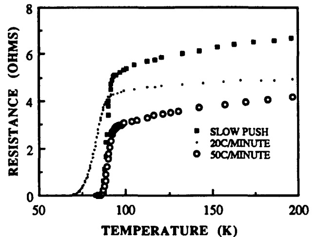
Figure 3: Resistance as a function of temperature for three samples on \text{SrTiO}_3 substrates with different annealing cycles. \text{Cu}/\text{Y}=3.00 , \text{Ba}/\text{Y}=2.25 . Annealed 45 minutes at 900^\circ\text{C} .
