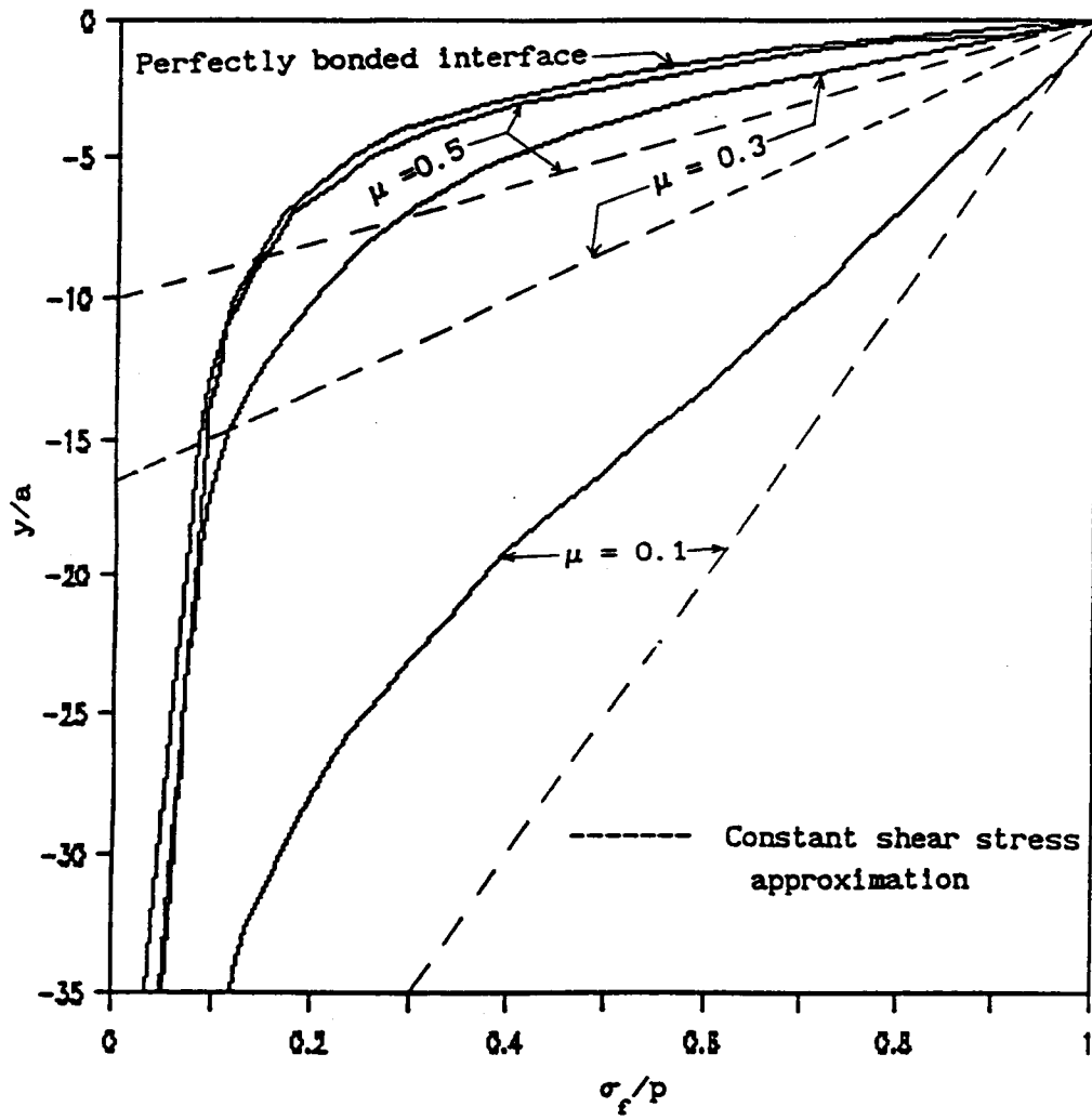
Fig. 10. Fiber load diffusion for compressive loading ( p/\sigma_0 = -5.0 ).
