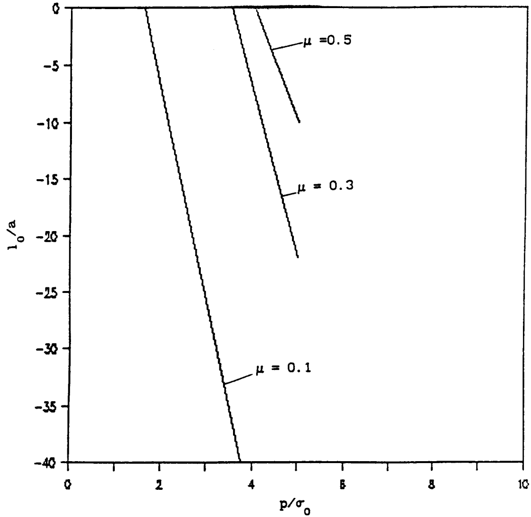
Fig. 7. Extent of delamination l_0 as a function of the normalized tensile load p/\sigma_0
