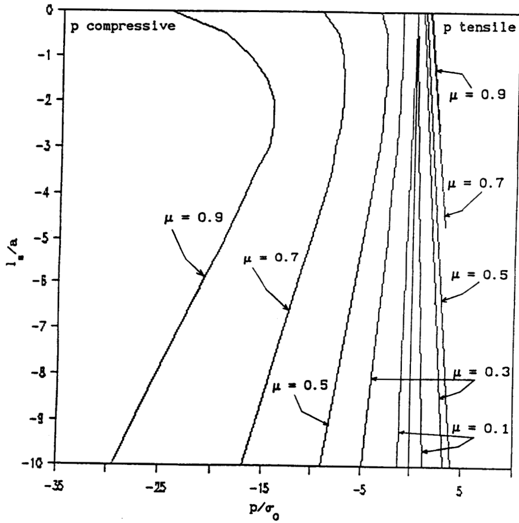
Fig. 6. Extent of slip as a function of the normalized load p/\sigma_0 .
