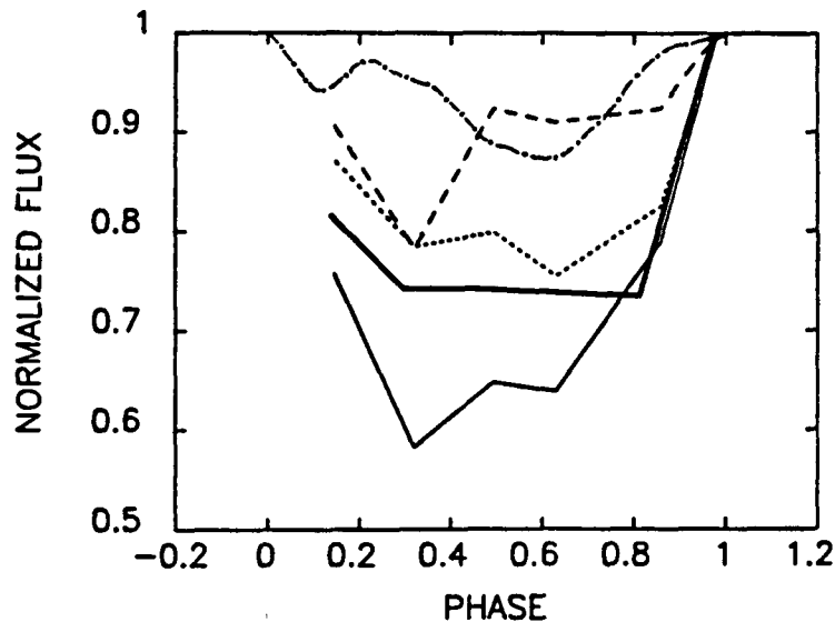
Figure 4: The magnetic flux ( \propto f_B , heavy solid), various ultraviolet emission line fluxes (C IV, solid; C II, dashed; O I, long dashed) and the smoothed, Ca II excess flux (dash-dotted) of \xi Bootis A, normalized and plotted versus rotational phase.
