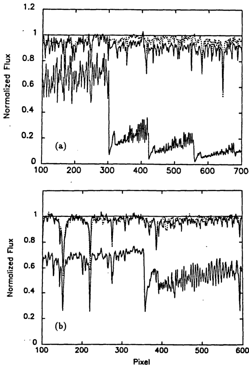
Figure 1. The 7100 Å (a) and 8860 Å (b) spectral regions of the K5Ve flare star BD +26°730 (upper solid curves), the photospheric proxy ξ Boo B (K4V; dashed curves), and the starspot proxy 2 Cen (M4.5III; lower solid curves). Note the excess absorption in the BD +26°730 spectra at the wavelengths of the TiO bands (which are clearly visible in the 2 Cen spectra). We derive T_{spot} = 3500 \pm 150 K and A = 0.20 \pm 0.04 .
