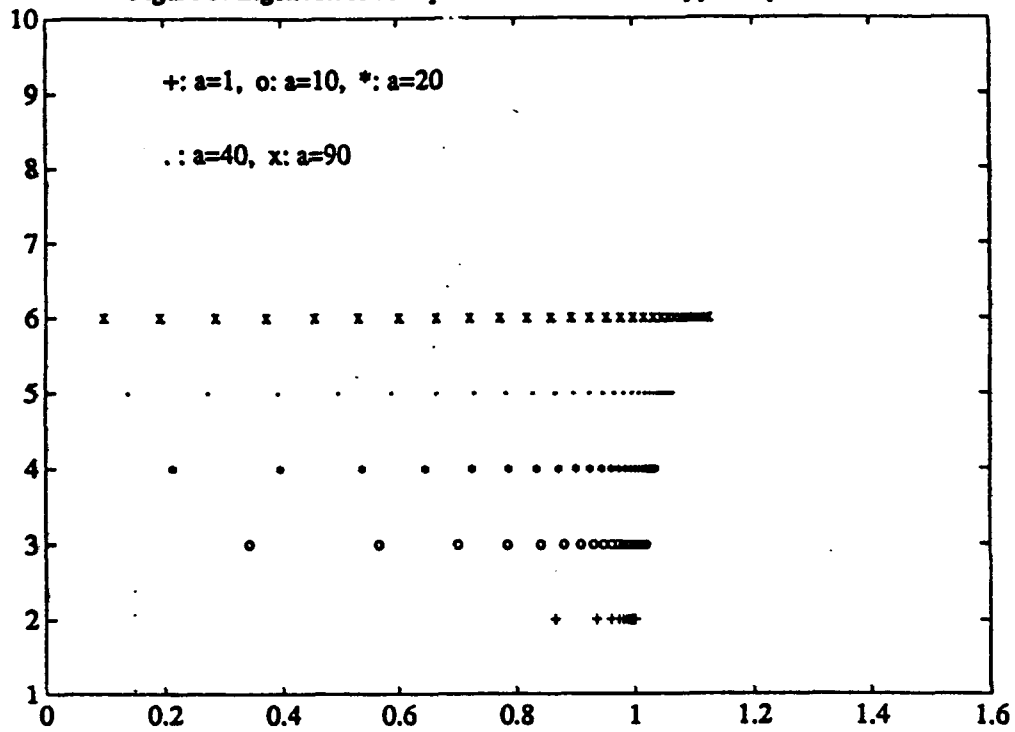
Figure 5. Eigenvalues for upwind diff. for U_{xx}+U_{yy}+a U_y=0 , h=0.02
