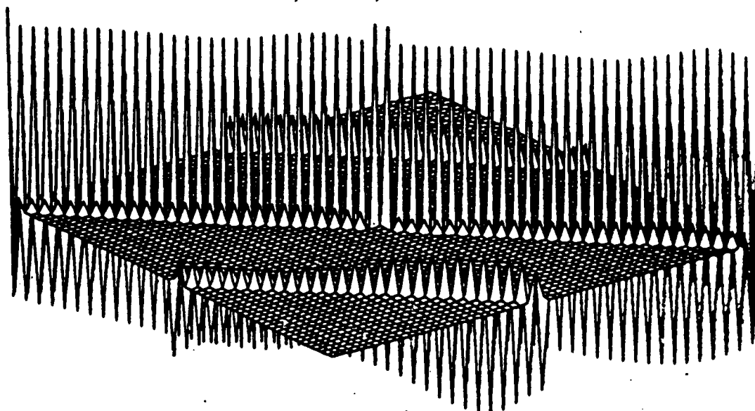
FIGURE 7 Plot of S , n=30 , R=200
