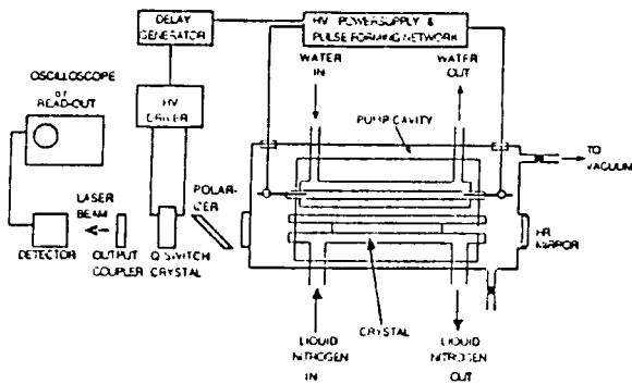
Fig.3 Schematic diagram for the experimental setup.
