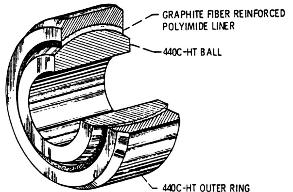
Figure 12. - Test bearings employing graphite fiber reinforced polyimide.
