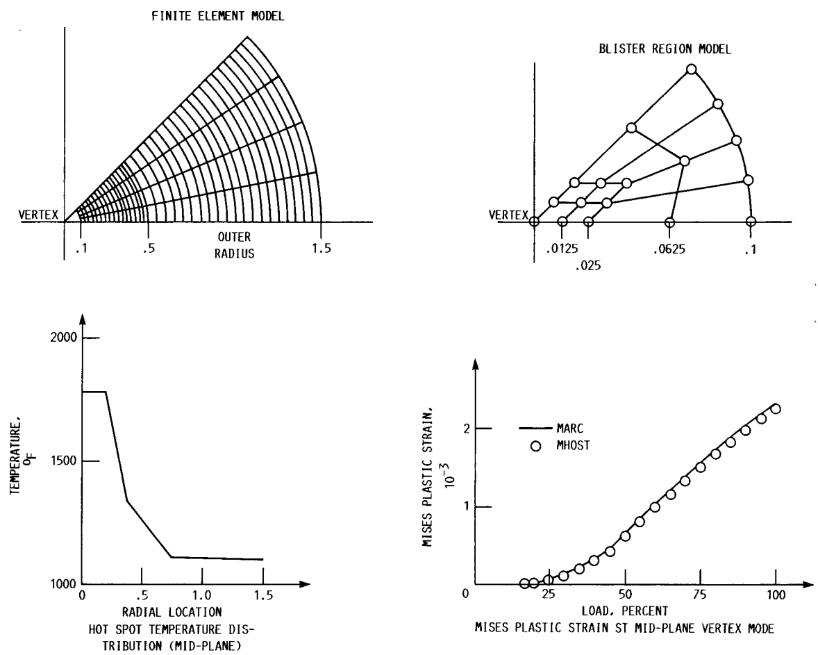
FIGURE 5. - BURNER BLISTER MHOST ANALYSIS. -
