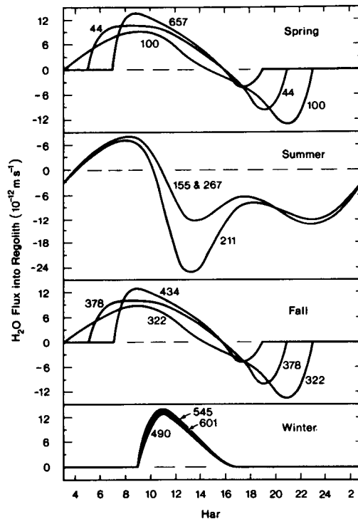
Figure 3. Diurnal cycles of H 2 O exchange with the Martian regolith. Illustrative example with DSF = 195 K. Note that 24 hars (Martian hours) = 1 sol. Numerals on curves show sol number, with sol 0 at vernal equinox.
