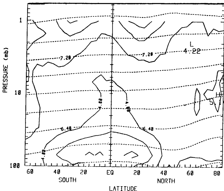
Fig. 1. Zonal mean LIMS water vapor concentration (ppmv) averaged for Jan. 10-15, 1979 superimposed on potential temperature (In(°K), dashed).
