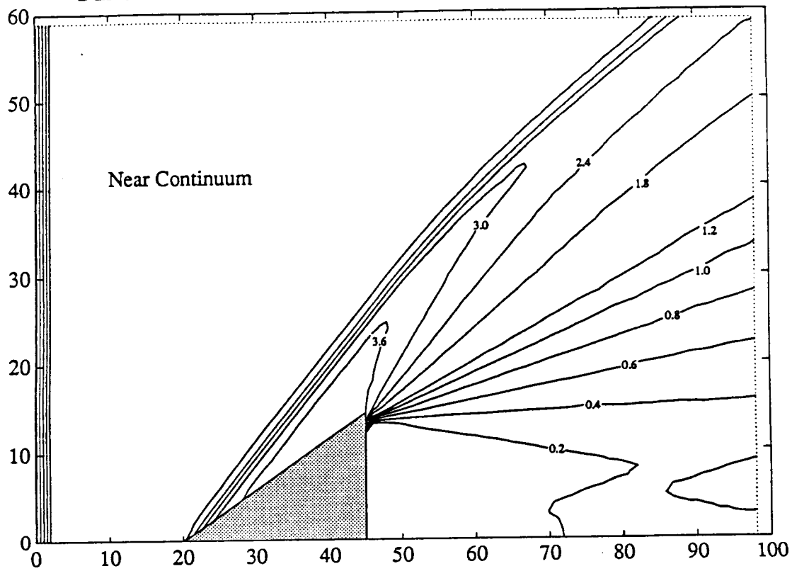
Figure 1. Density contours for near continuum Mach 4 flow over a 30° wedge.
