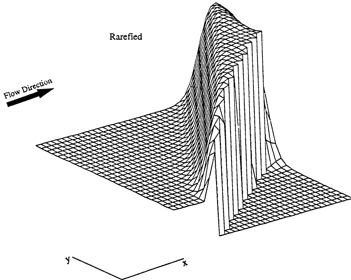
Figure 6. Density surface in the stagnation region for rarefied Mach 4 flow over a 30° wedge. The freestream mean free path is 0.5 cell widths, corresponding Knudsen and Reynolds number are 0.02 and 600 respectively.
