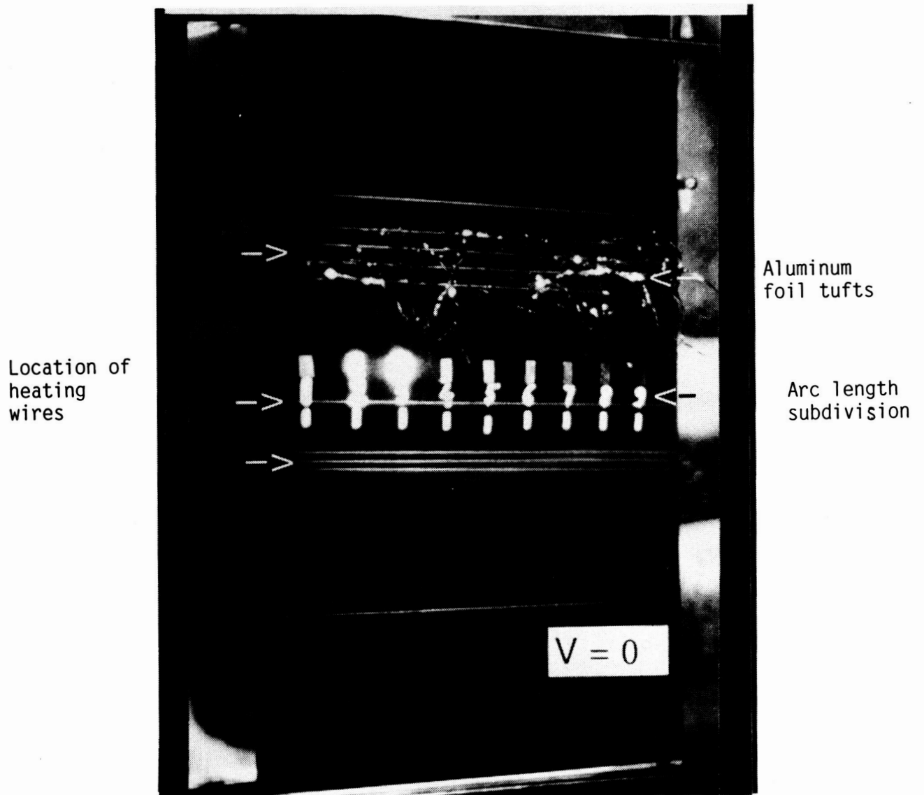
Fig. 6.2 NACA 0012 airfoil with aluminum foil tufts in still air.
