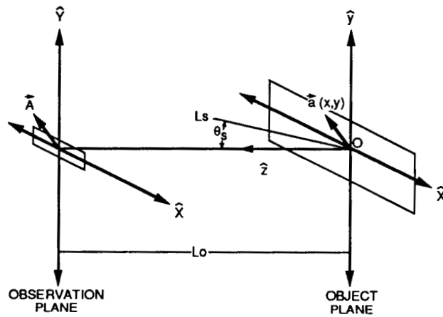
Figure 3.1.1. - Simplified coordinate system.
