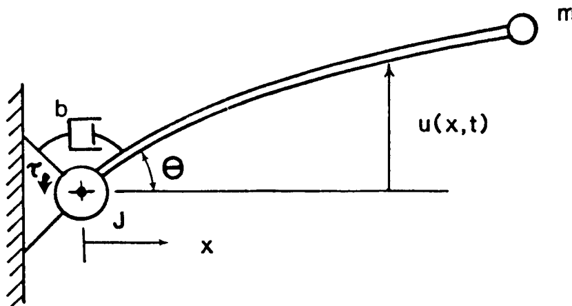
Figure 1. System Configuration
