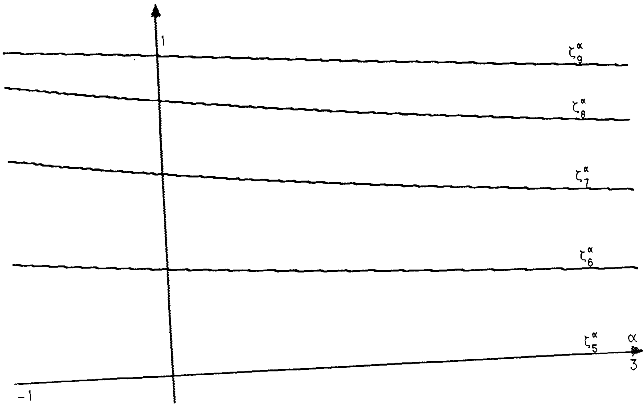
Figure 2 The five nonnegative zeros of J_9^\alpha as a function of \alpha .
