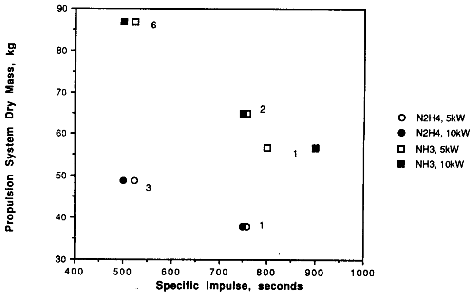
Figure 8. - Arcjet propulsion system dry masses versus specific impulse. Number of thrusters is indicated.
