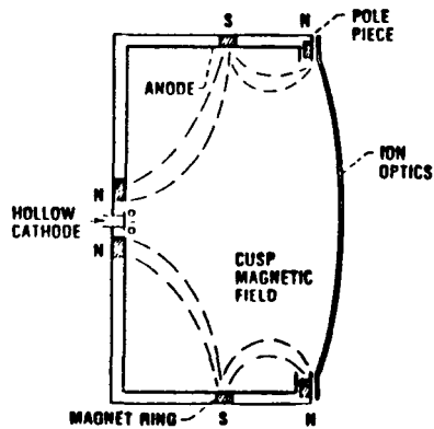
Figure 1. - Cross section of ring-cusp ion thruster.
