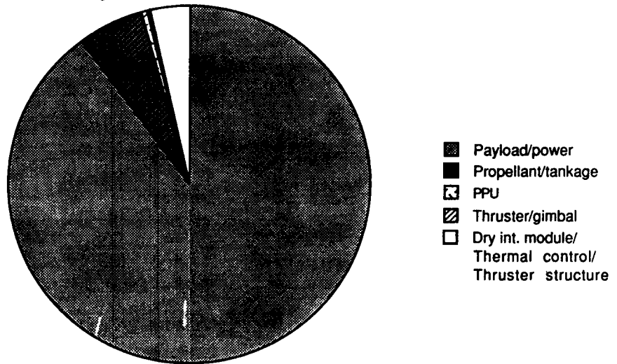
Figure 12. - Spacecraft mass distribution with 2-engine 10kW Xe ion option. 5000 hour thrusting time. Total s/c mass 3283 kg. Mission Mode II
