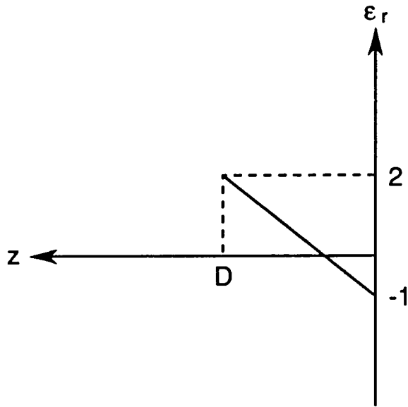
Figure 2.-Linear profile.
