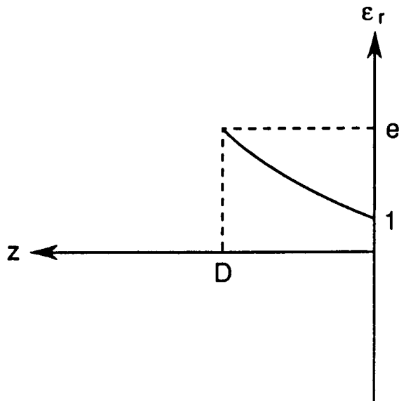
Figure 3.-Exponential profile.
