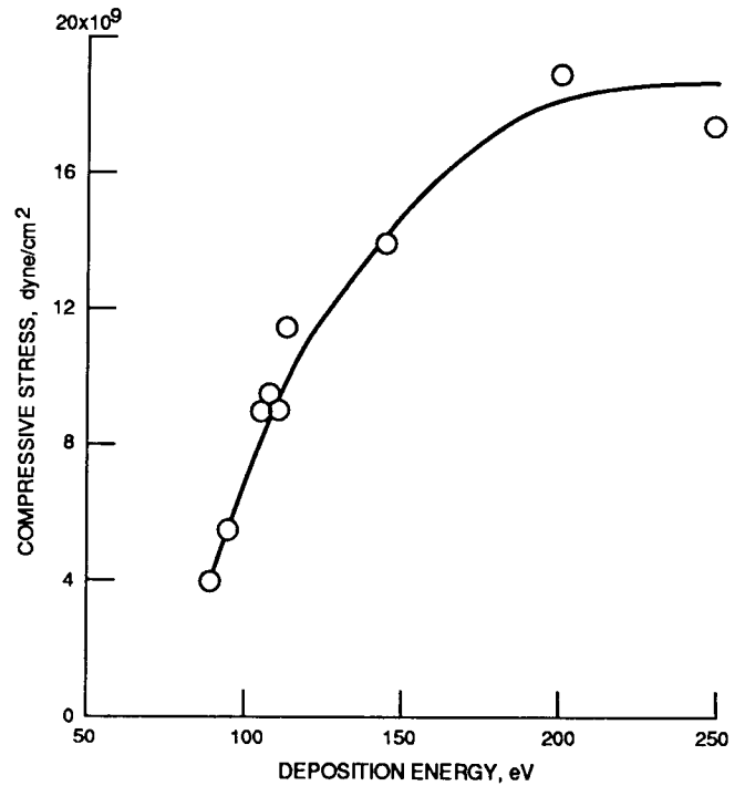
Figure 2. - Compressive stress as function of deposition energy for 0.1- \mu m-thick DLC films made with CH 4 in the single ion-beam source.
