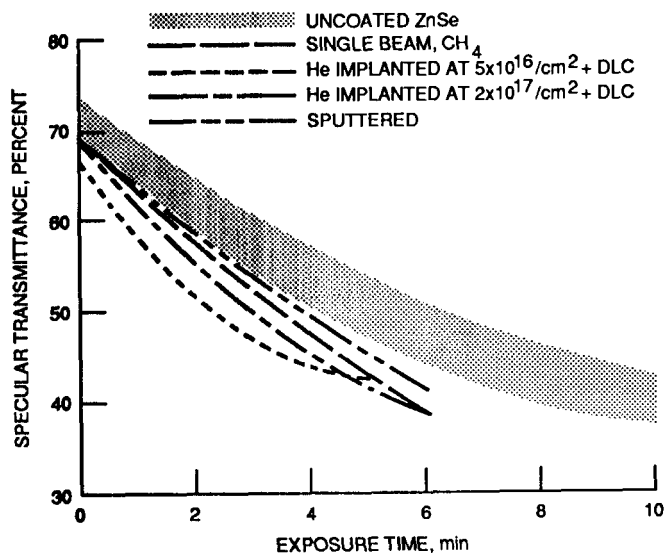
Figure 11. - Change in specular transmittance at 10 \mu\text{m} due to total erosion time for various surfaces of ZnSe coated with DLC films.
