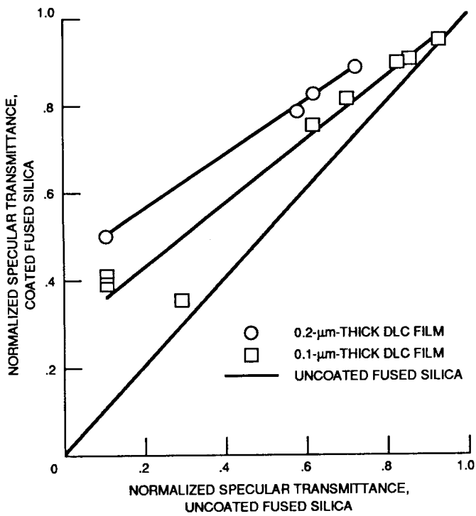
Figure 8. - Normalized specular transmittance of fused silica coated with DLC films, 0.1 and 0.2 \mu\text{m} thick, made with \text{CH}_4 in the single ion-beam source, and uncoated fused silica, both after exposure to 100- \mu\text{m} \text{SiO}_2 particles at 27 m/sec.
