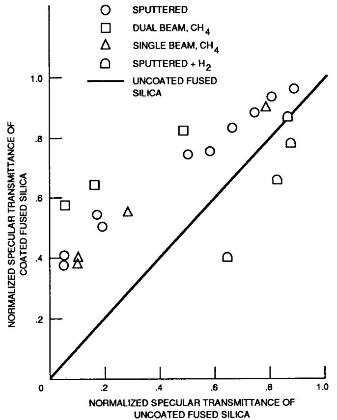
Figure 9. - Protection that 0.1- \mu\text{m} -thick DLC films deposited by various methods afforded fused silica after exposure to 100- \mu\text{m} \text{SiO}_2 particles at 27 m/sec.
