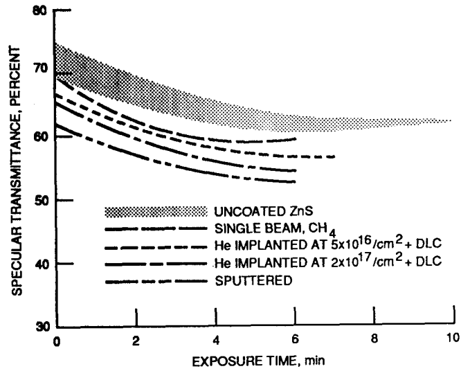
Figure 10. - Change in specular transmittance at 10 \mu\text{m} due to total erosion time for various surfaces of ZnS coated with DLC films.
