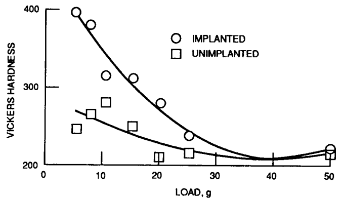
Figure 4. - Vickers hardness as function of applied load for unimplanted ZnS, and for ZnS implanted with He ions, at 100 keV at a dose of 2x10 17 particles/cm 2 .
