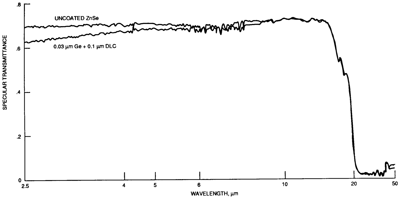
Figure 7. - Specular transmittance of 0.1- \mu\text{m} DLC film made with \text{CH}_4 in the single beam with and without an intermediate layer of 0.03- \mu\text{m} Ge on the ZnSe substrate.
