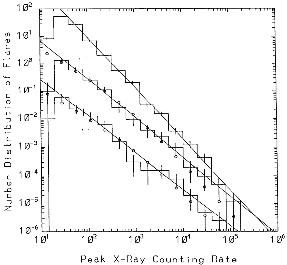
Fig. 2. Distribution of all HXRBS events N_o(X) and N_{R_o}(X) for R_o = 75 and 300 with the R_o = 300 histogram reduced by a factor of ten for clarity. The solid lines show the best fit power-law for each of the histograms. The circles are the values calculated using the best fit to the function G(Y) .
