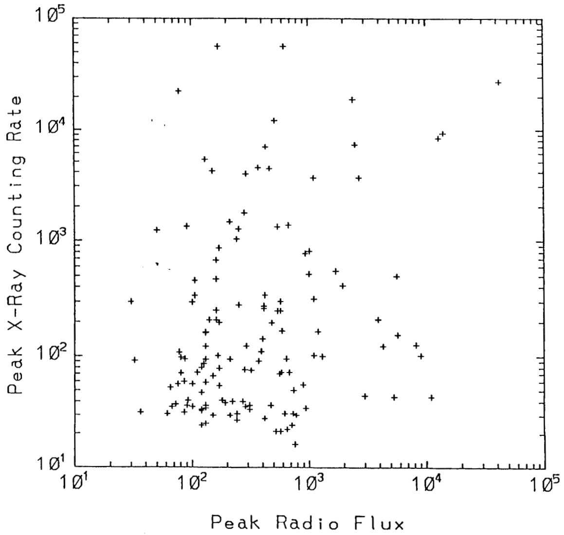
Fig. 1. Distribution of the correlated events in the R-X plane.
