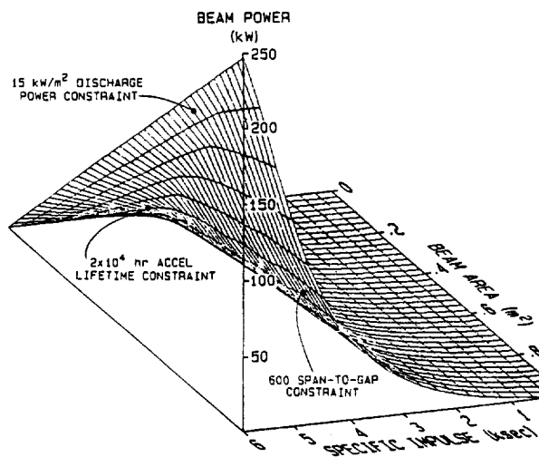
Fig. 10. Typical Overall Power Constraining Surface (Span-to-Gap, Discharge Power and Accel Grid Life Limiting)
