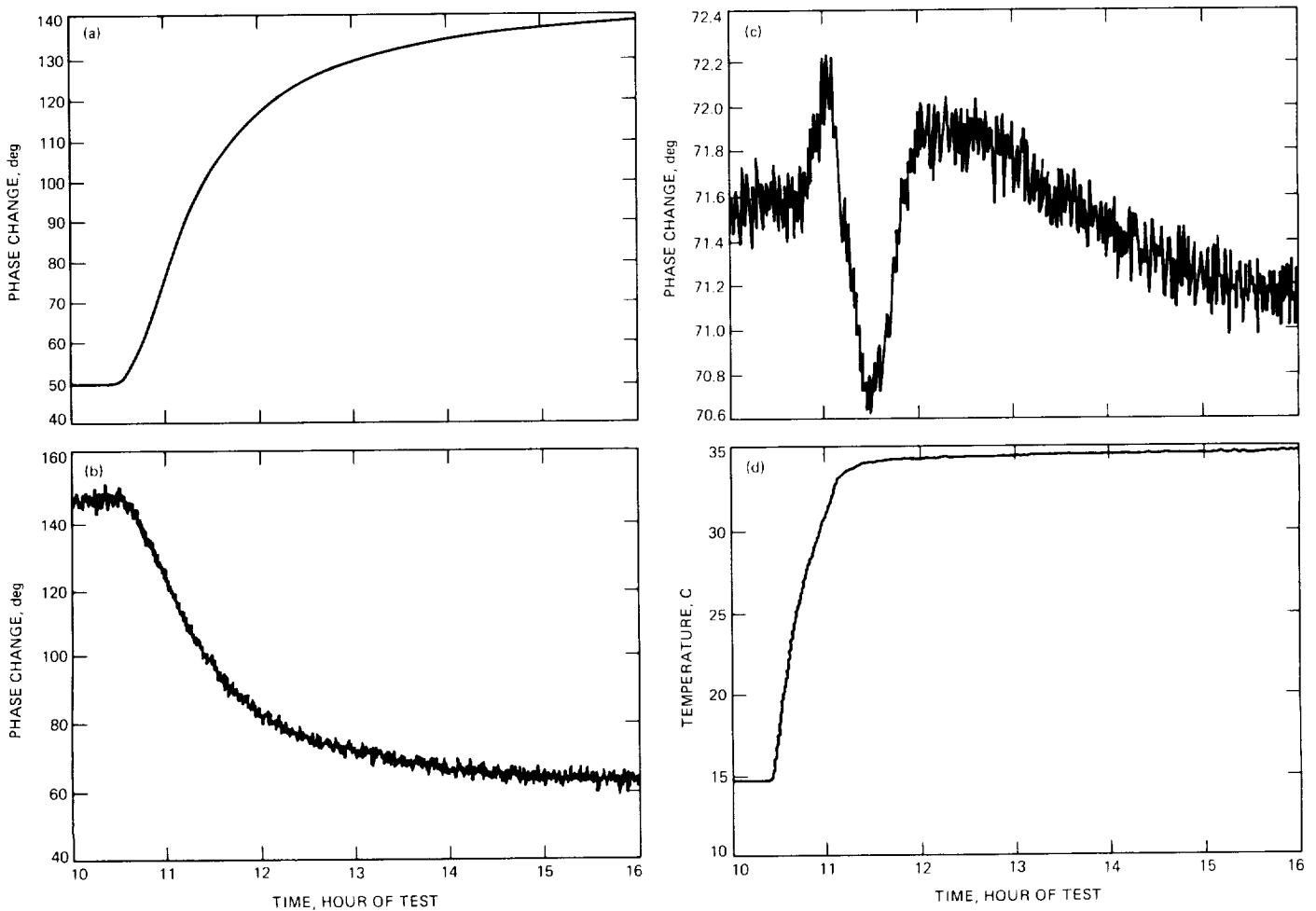
Fig. 7. Fiber-optic test results, phase step change in temperature 15 to 35 °C: (a) reference unit (near-end) transmitter; (b) reference unit (near-end) receiver; (c) remote unit (far-end) receiver; (d) test chamber temperature.
