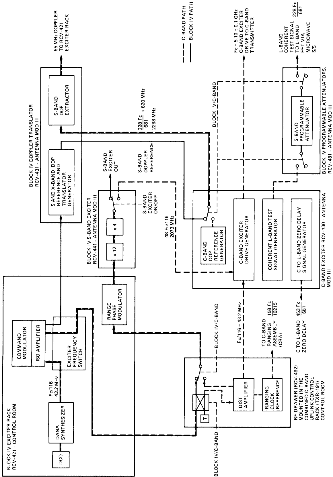
Fig. 1. Block IV receiver-exciter and C-band exciter interfaces.
