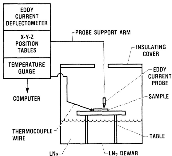
FIGURE 1. - DIAGRAM OF EXPERIMENTAL SETUP.
