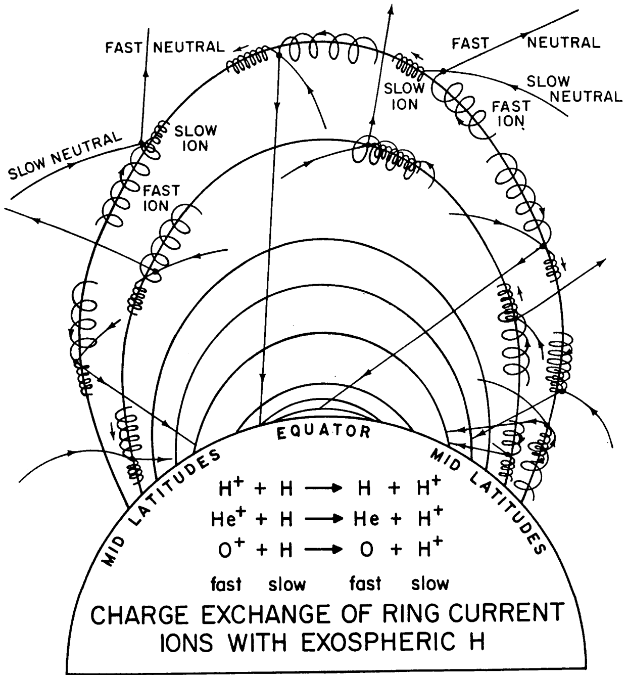
Figure I-13. Geometry of the production of energetic neutral atoms of H, He, and O from the corresponding trapped ions H^+ , He^+ , and O^+ in the ring current.
