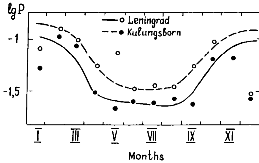
Figure 5. Seasonal variations of the fraction of time when SPA were observed [Danilov et al., Geomagnetism i aeronomia , 27, 536, 1987].
