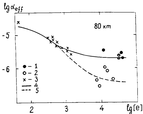
Figure 3. The effective recombination coefficient \alpha_{\text{eff}} versus the electron concentration [e] at 80 km according to Danilov and Simonov [in Ionosfernye issledovania , N 34, 54, 1981]: 1 – PCA, summer 1972; 2 – PCA, winter 1969; 3 – solar eclipses 1969 and 1970; 4 and 5 – theoretical curves (taking into account the dependences of \alpha_{\text{eff}} on f^+ and f^+ on [e] and the season) for summer and winter, respectively.
