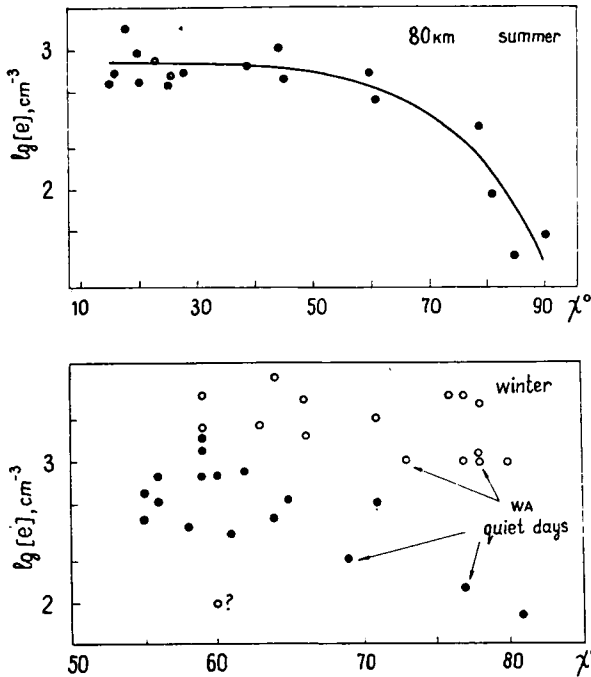
Figure 1. Electron concentrations as a function of solar zenith angle \chi according to Danilov et al. [in Spatial and Temporal Structure of the Lower Ionosphere , 1982]. The dark points are normal days, the open ones are winter anomaly days.
