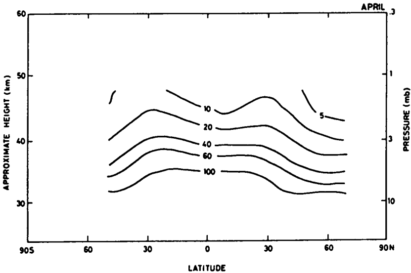
Figure 8. Monthly-averaged latitude-height cross section of N_2O volume mixing ratio (ppbv) for April 1979 from the SAMS satellite measurements [Gray and Pyle, Q. J. R. Met Soc. , 1986].
