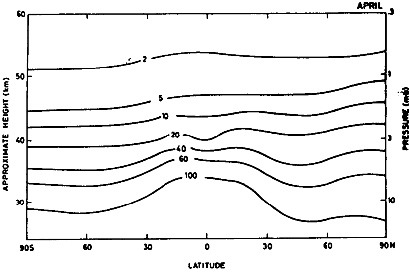
Figure 7. Monthly-averaged latitude-height cross section of N_2O volume mixing ratio (ppbv) for April from run B [Gray and Pyle, Q. J. R. Met Soc. , 1986].
