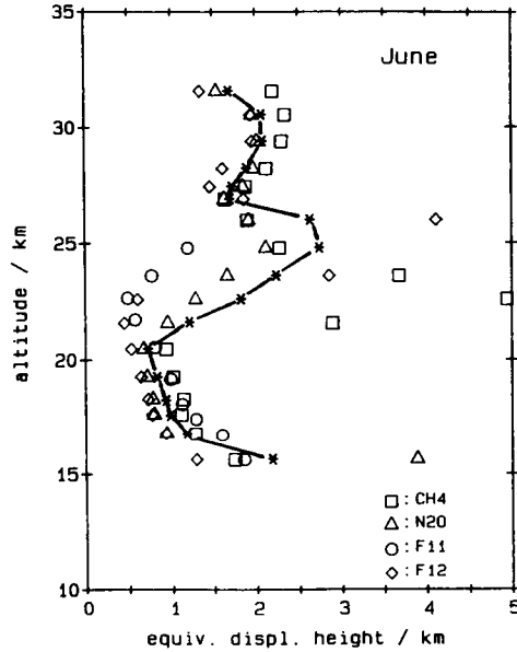
Figure 4. The vertical distribution of the equivalent displacement height, deduced from measurements of \text{CH}_4 , \text{N}_2\text{O} , and \text{CFCl}_3 , and \text{CF}_2\text{Cl}_2 . The balloons were launched during June (1977-1979). The heavy line runs through averages of the individual EDH. Values for \text{CFCl}_3 above 25 km were omitted.
