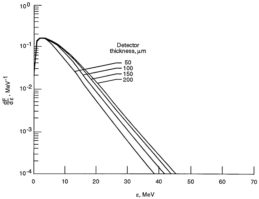
Figure 8. Total absorption spectrum for surface-barrier detector of 50 to 200 \mu\text{m} and E_0 = 3.5 MeV.
