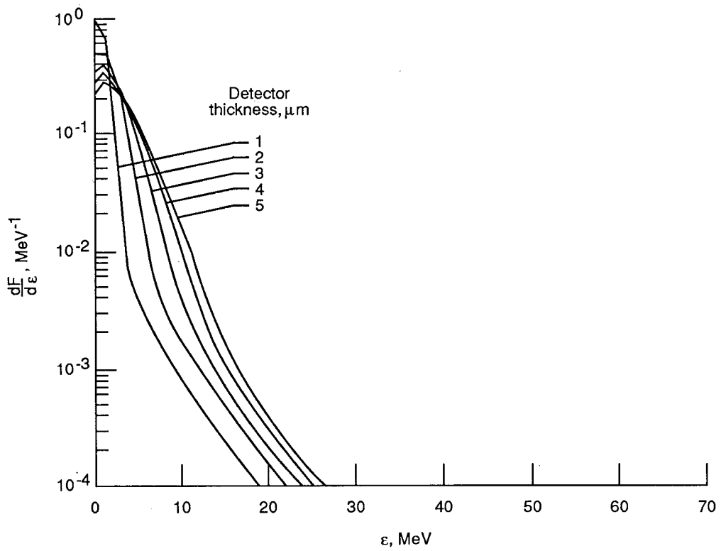
Figure 7. Total absorption spectrum for surface-barrier detector of 1 to 5 \mu\text{m} and E_0 = 3.5 MeV.
