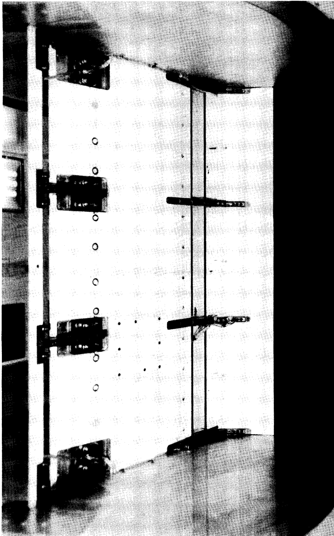
Figure 11.- Photograph of lower surface of small-vane model showing bracket arrangement. View looking downstream.
