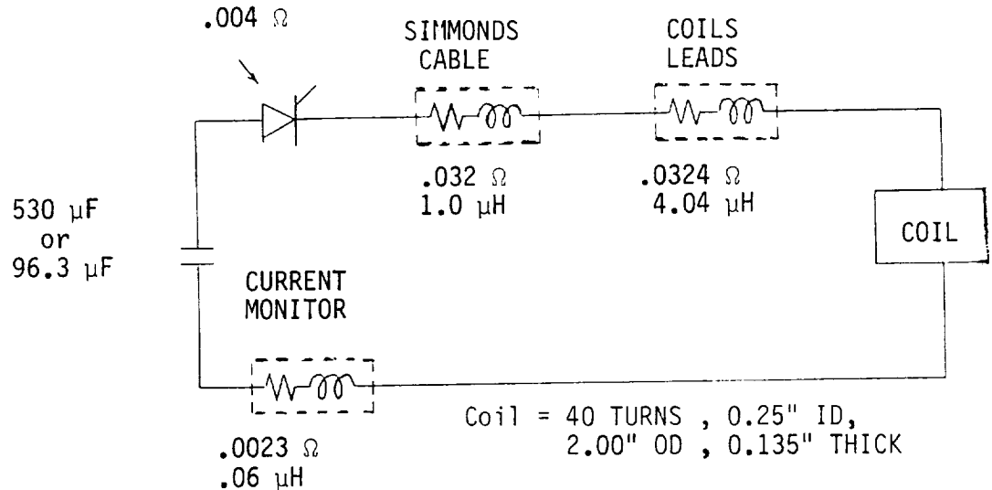
Fig. 2-73 Circuit Characterization for Lewis Experiment
