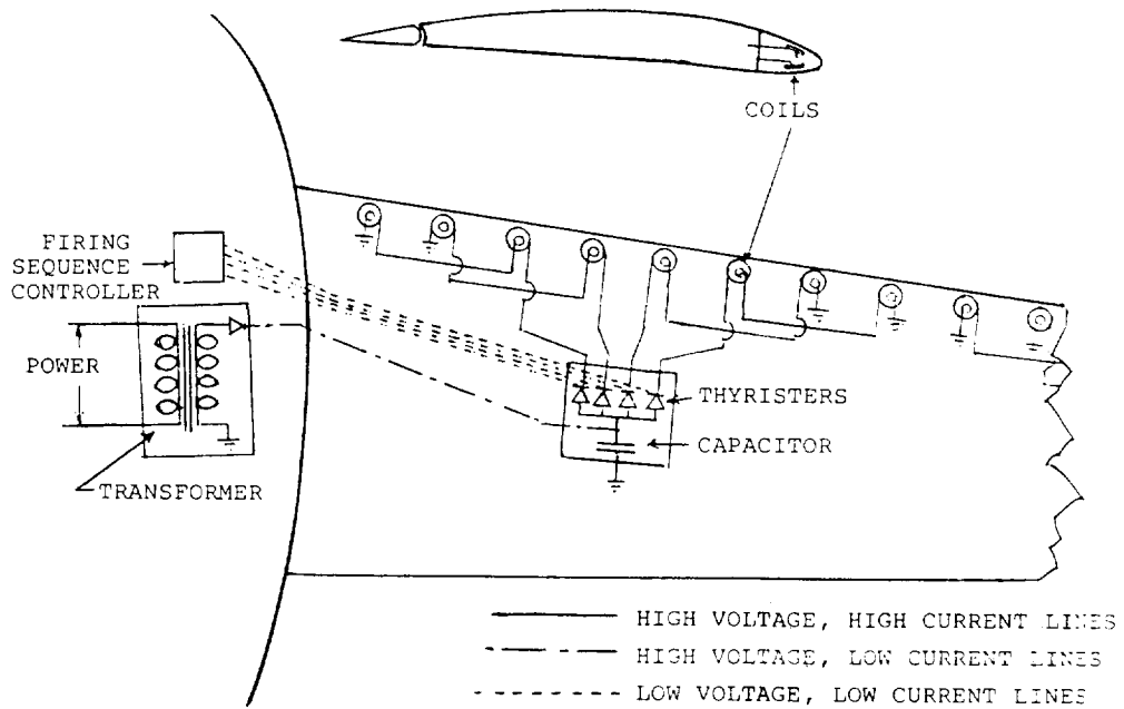
Fig. 1-6 EIDI with Series-Connected Coils ("Odds and Evens")
