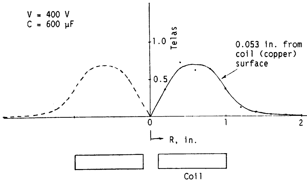
Fig. 2-20 Maximum B_r vs Radius, no Target Present
