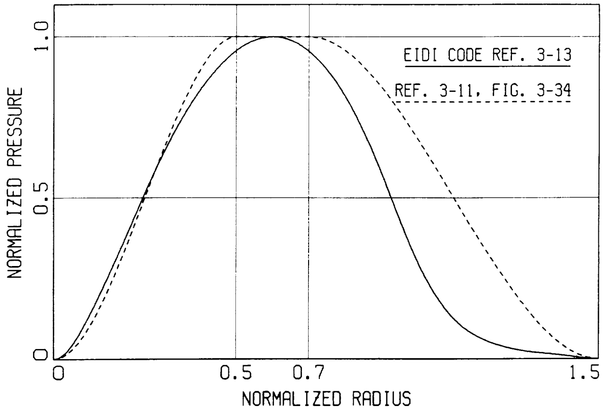
Figure 3-41 Normal Pressure Comparison
