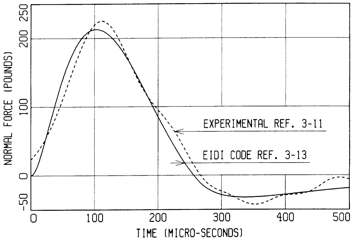
Figure 3-42 Normal Force Comparison Experimental Vs. EIDI Code
