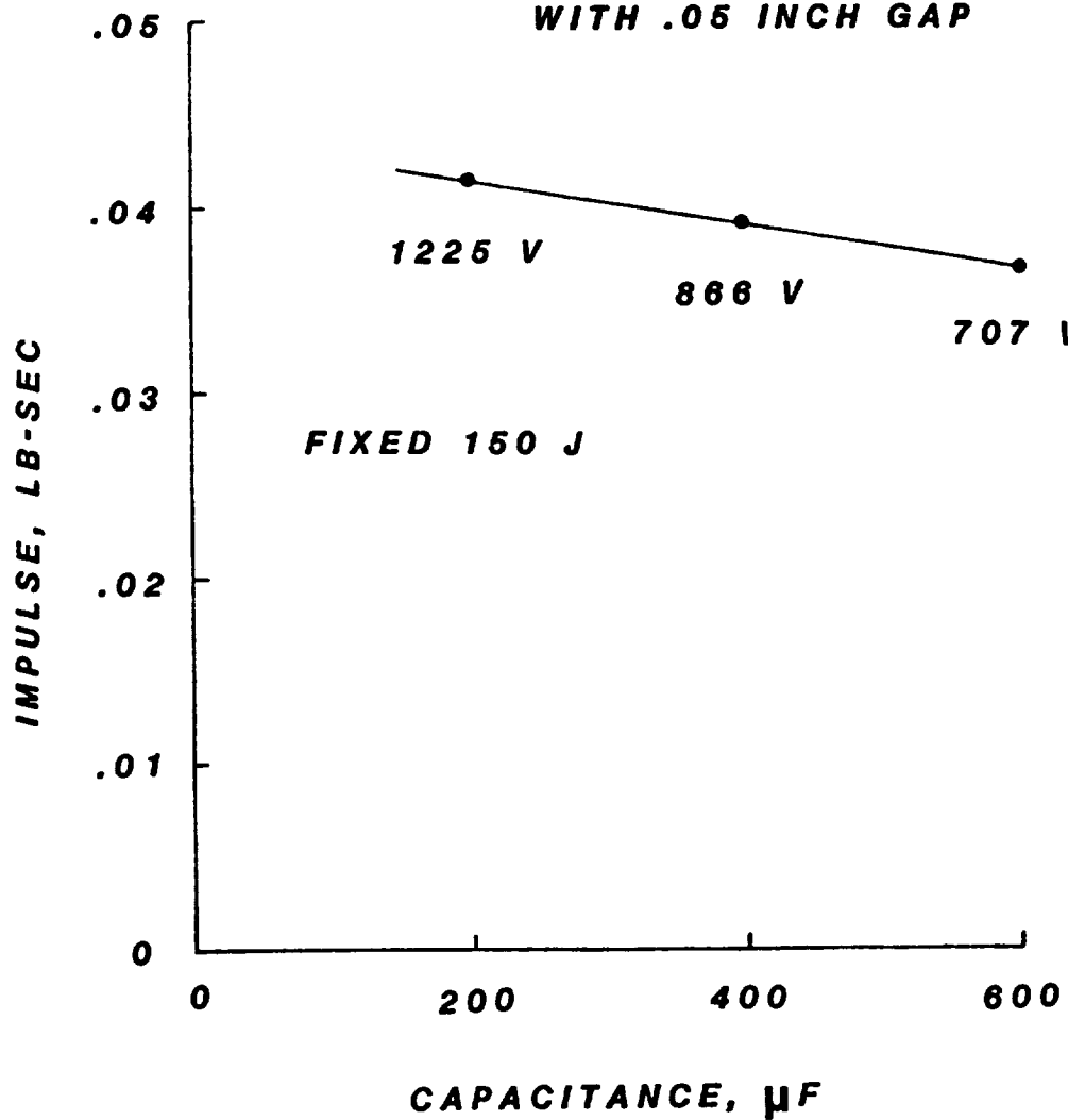
Fig. 2-6 Impulse vs Capacitance with Fixed Energy
