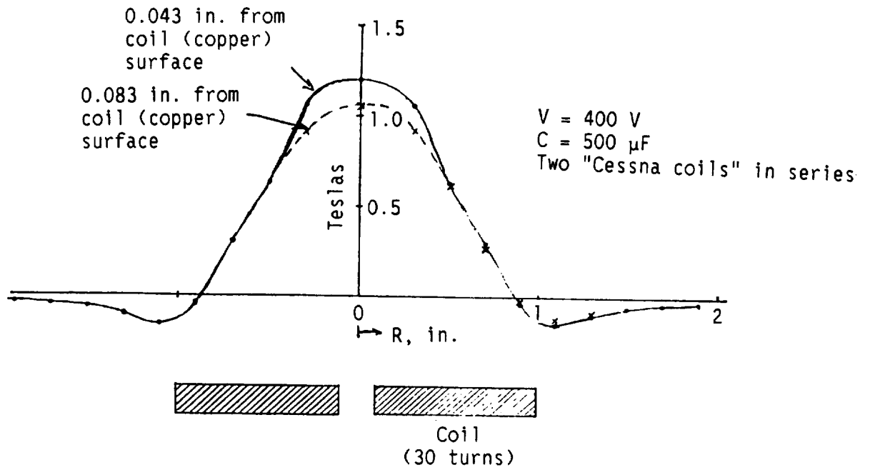
Fig. 2-19 Maximum B_L vs Radius, no Target Present
