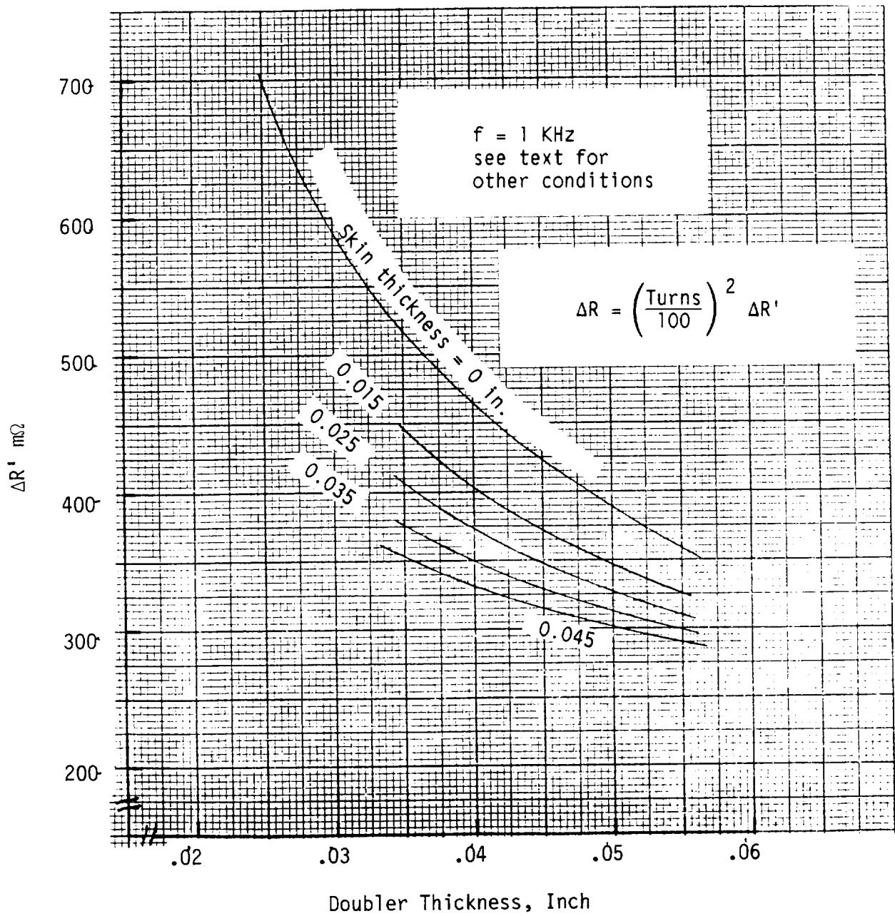
Graph 2-9b Effect of Doubler - Skin Combinations on Coil Resistance
