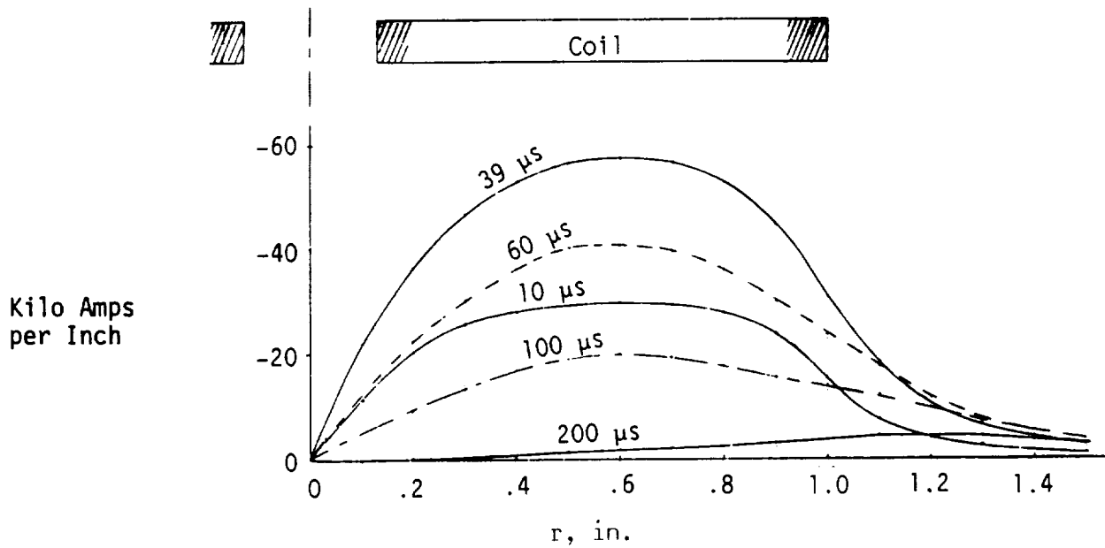
Fig. 2-81 Eddy Current Density, dI/dr
