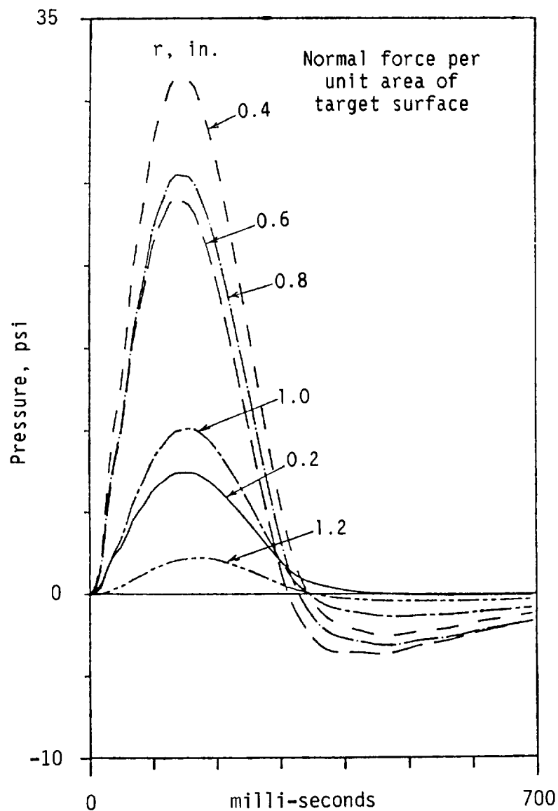
Fig. 2-30 Pressure vs Time at Various Radii
