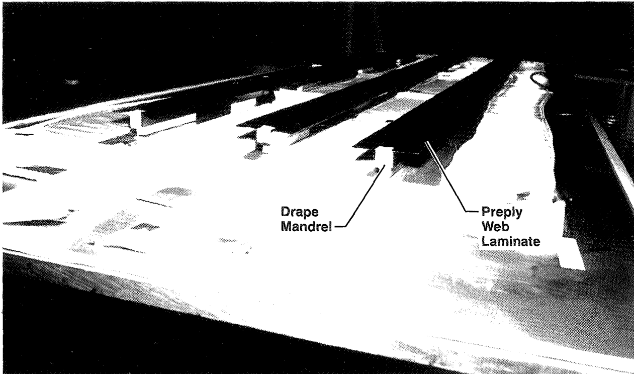
Figure 72. Stringer Web Preplies Prior to Heat-Assisted Drape Forming (Tests 3 and 4)
