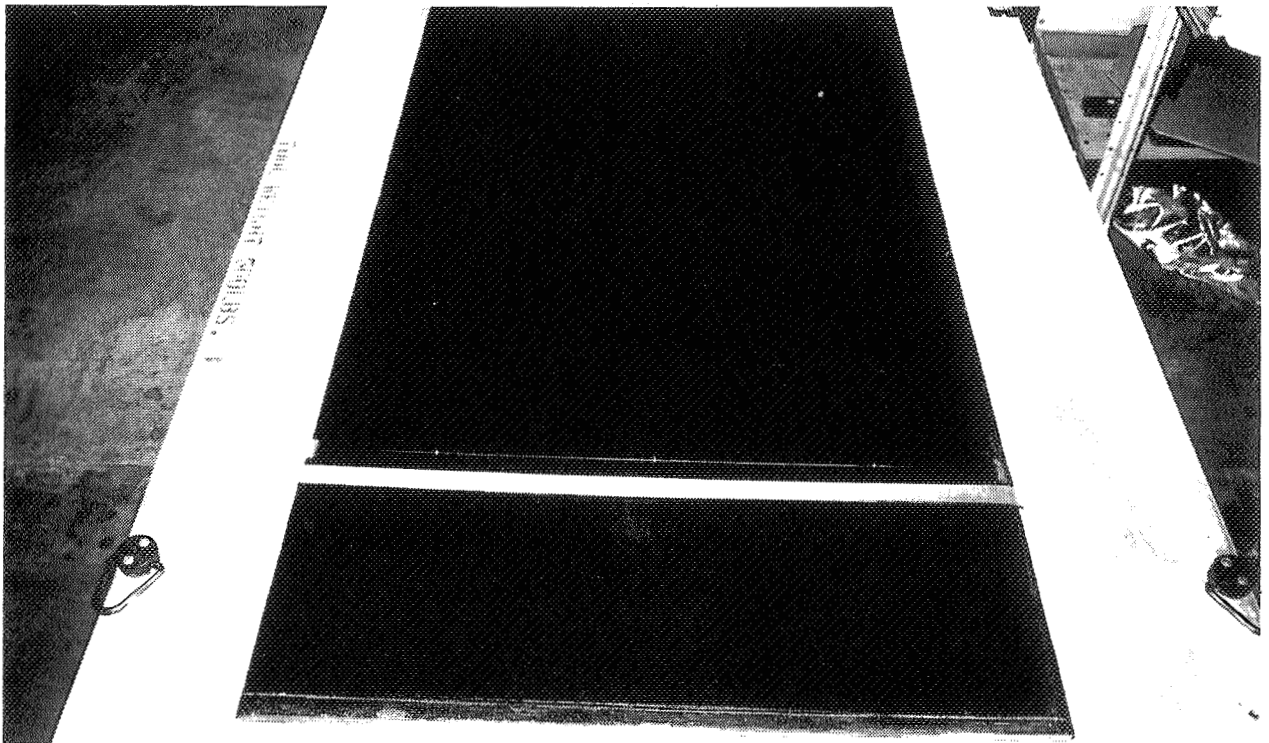
Figure 77. Cured 30-in by 100-in Panel Prior to Application of Grip Doublers (Test 1B)
