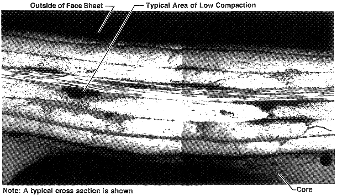
Figure 25. Photomicrograph of the Ciba-Geigy 2566/AS6 Material System
