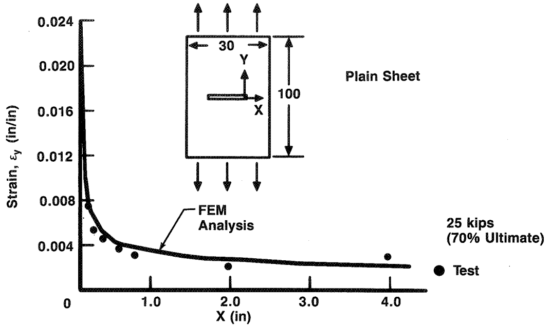
Figure 96. Predicted and Test-Derived Strains Near Damage Tip in an Unstiffened Fracture Panel (Test 1A-1)
