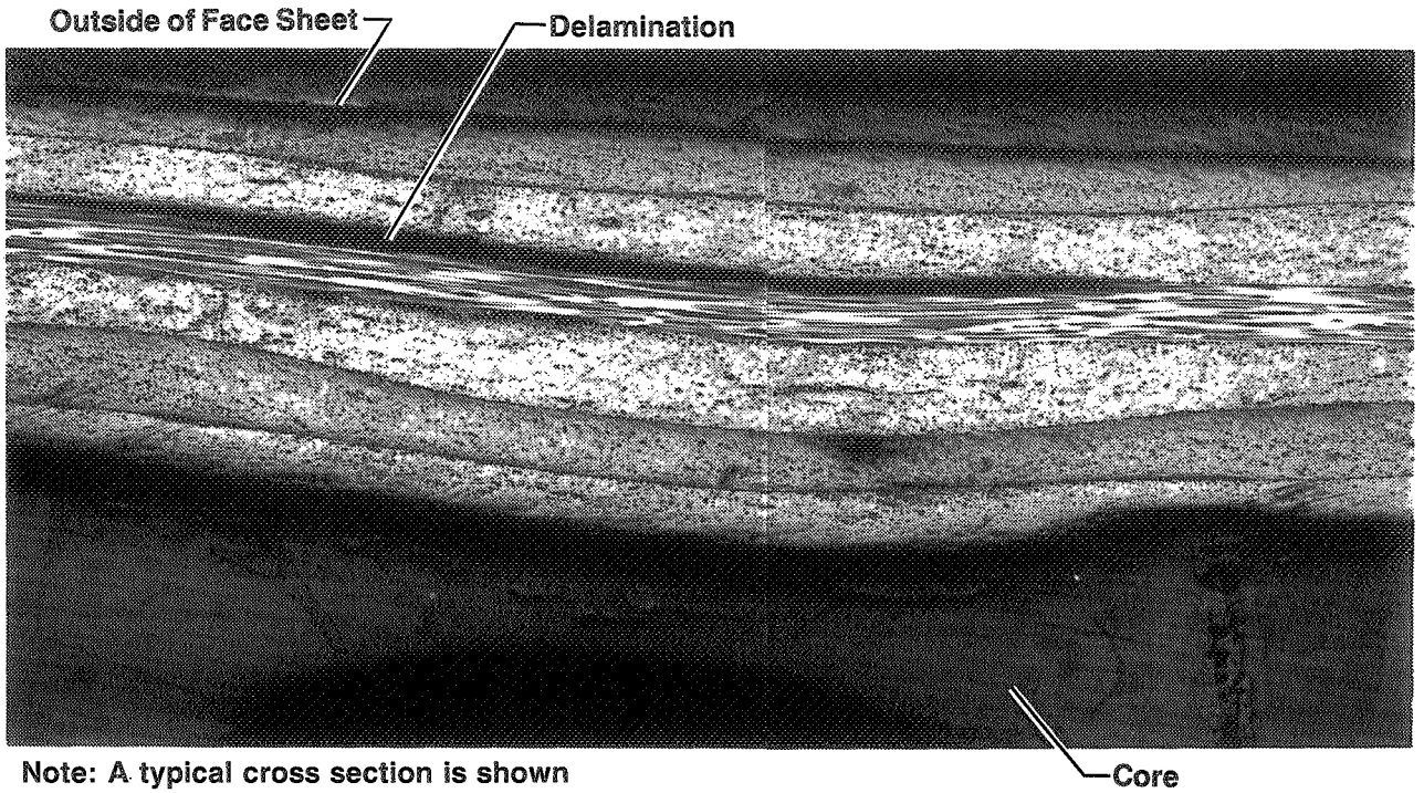
Figure 24. Photomicrograph of the Hercules 2220-3/AS6 Material System
