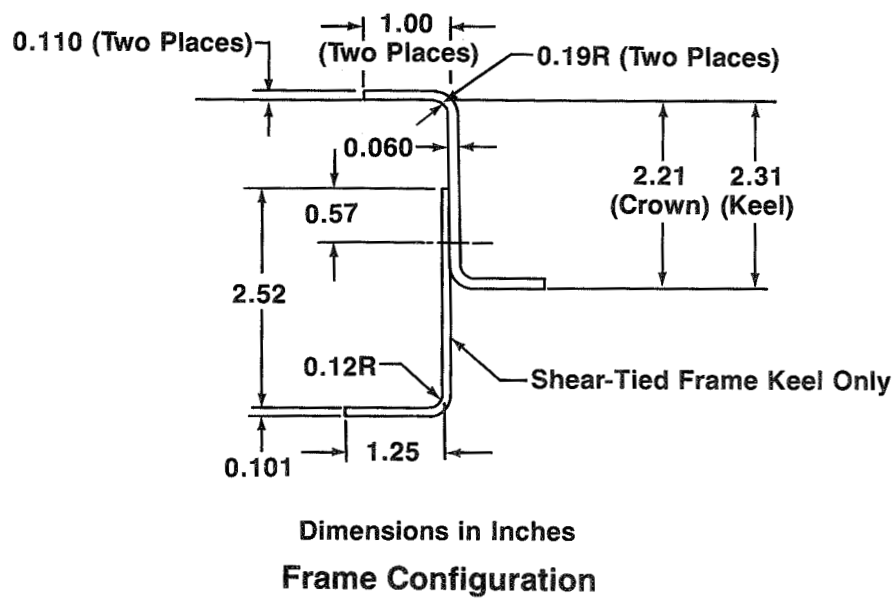
Figure 37. Frame Configuration for Fuselage Section Design
