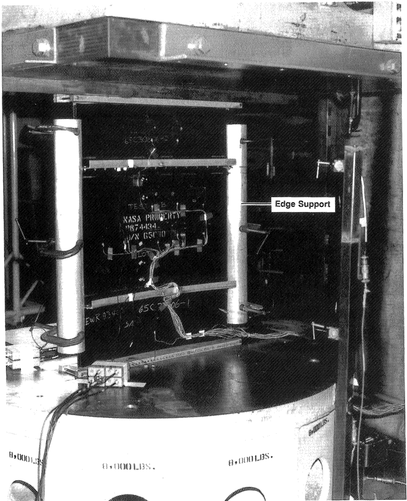
Figure 157. Honeycomb Compression Panel Test Setup (Test 6B)
