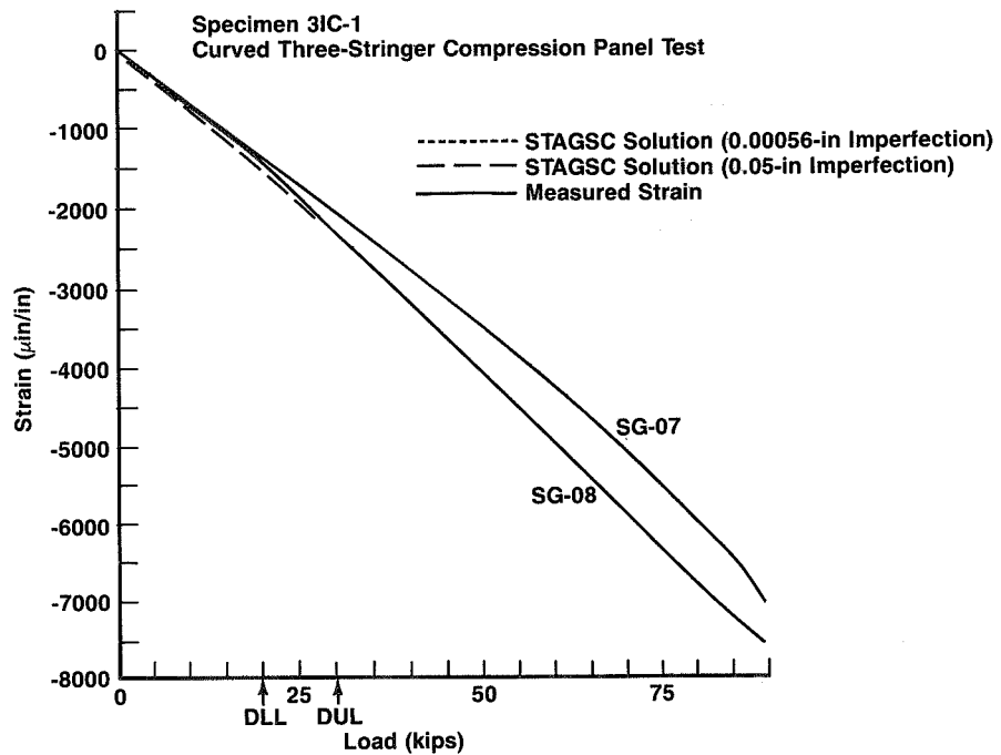
Figure 134. Measured and Predicted Strains in Center Stringer Web and Cap of Crown Compression Panel 4C-1
