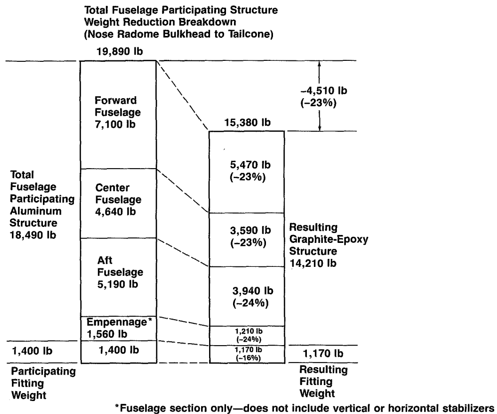
Figure 41. Weight Reduction of Fuselage Study Section
