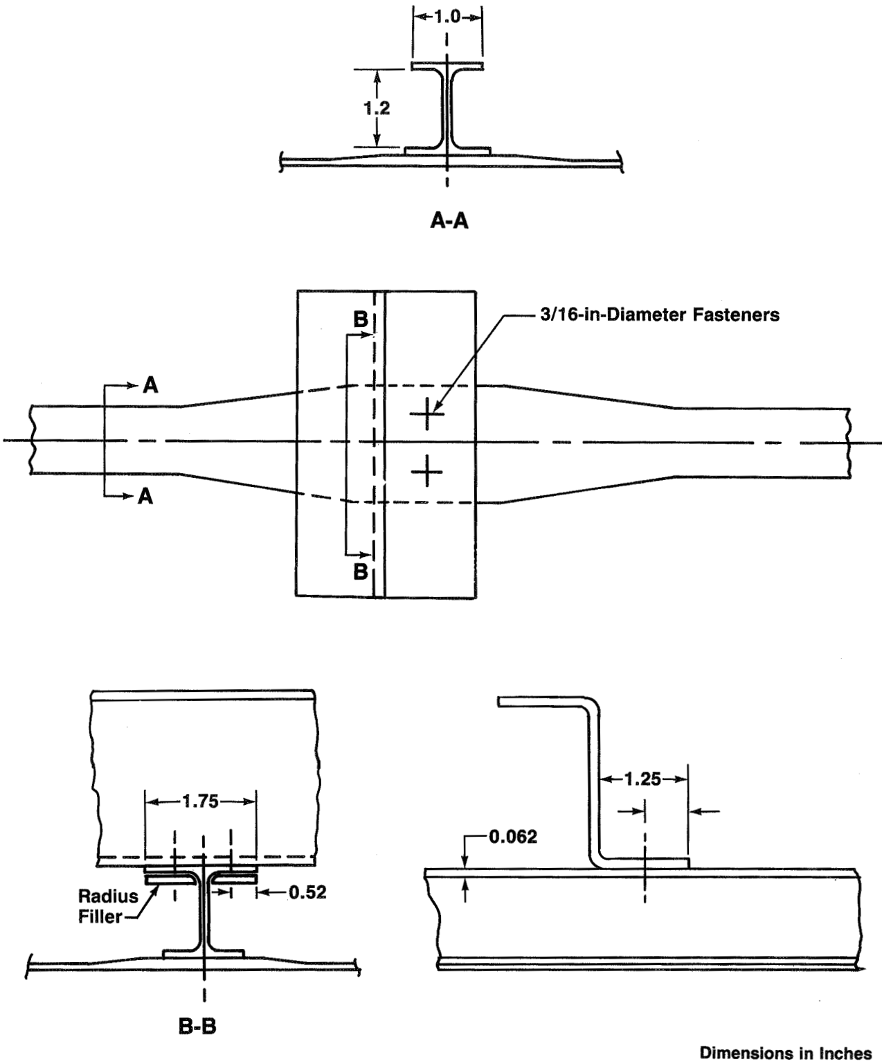
Figure 31. Typical Body Frame-to-Stringer Attachment
