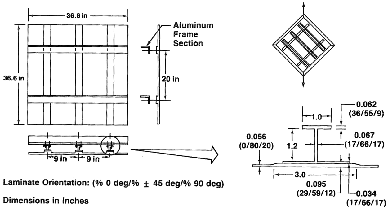
Figure 137. Skin-Stringer Shear Panel Configuration (Test 5)
