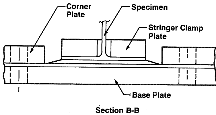
Figure 167. Fixture for Pressure Pilloving Panel Tests (Test 7)
