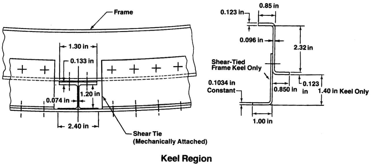
Figure 13. Concept 2—Laminate Skin With I-Section Stringers
