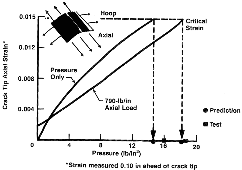
Figure 111. Curved Fracture Panel Failure Analysis
