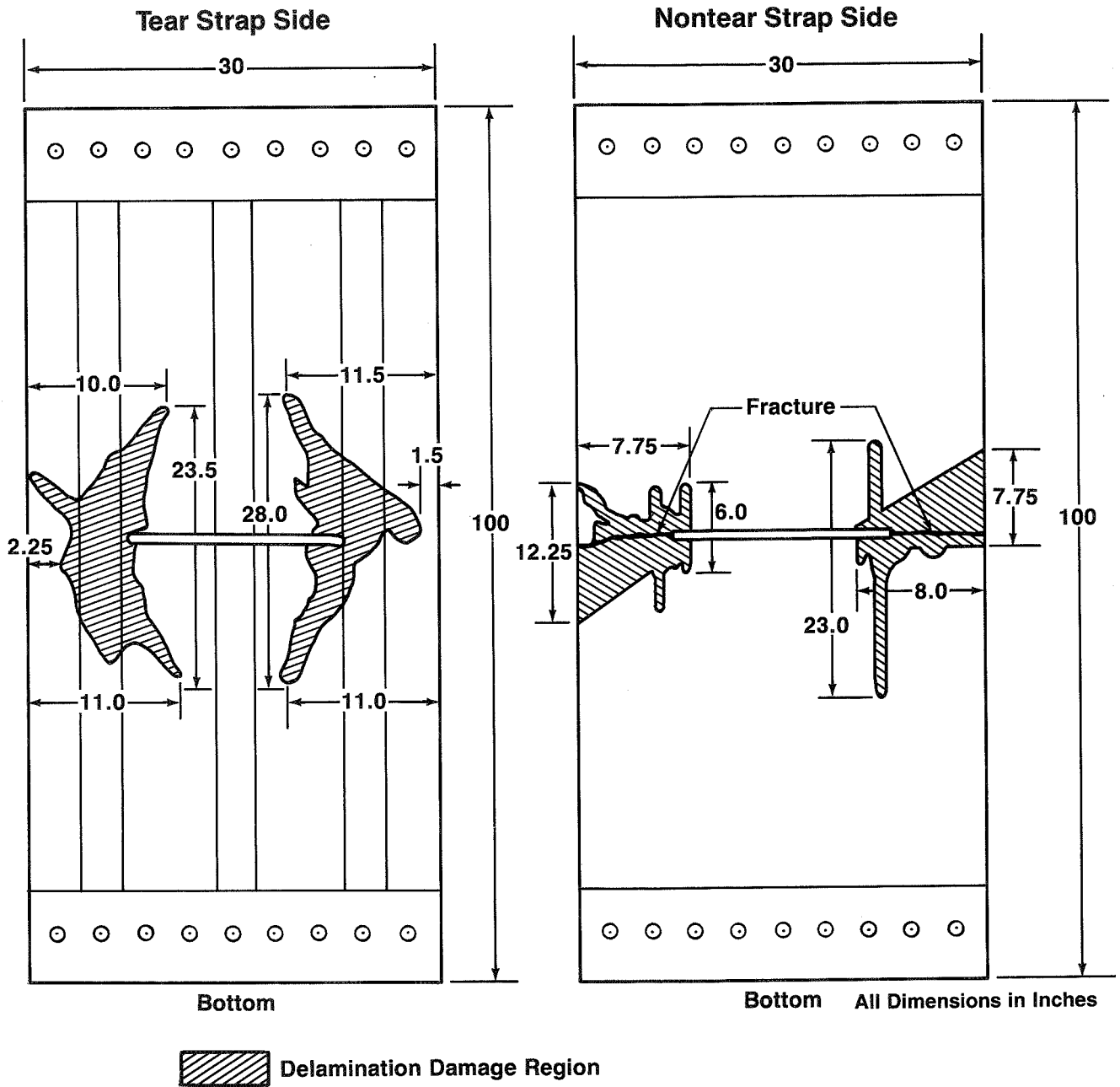
Figure 102. Postfailure Pulse Echo Inspection of the -2 Panel (Test 1B)
