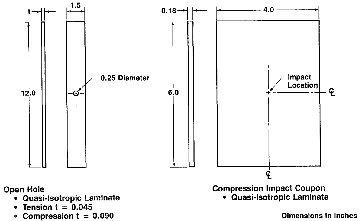
Figure 20. Open-Hole and Compression Impact Coupons
