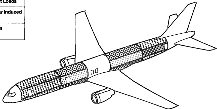
Figure 2. Critical Load Conditions for Pressure-Damage-Tolerant Design
