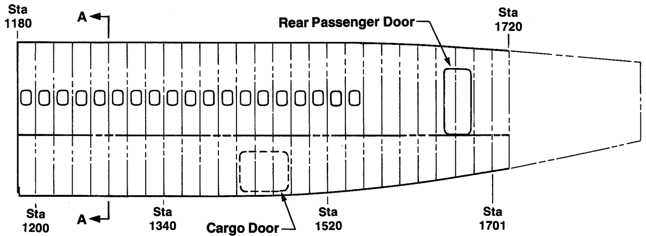
Figure 6. Fuselage Study Section
