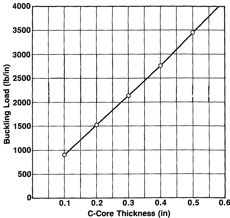
Figure 11. Buckling of Curved Honeycomb Fuselage Skin Panels
