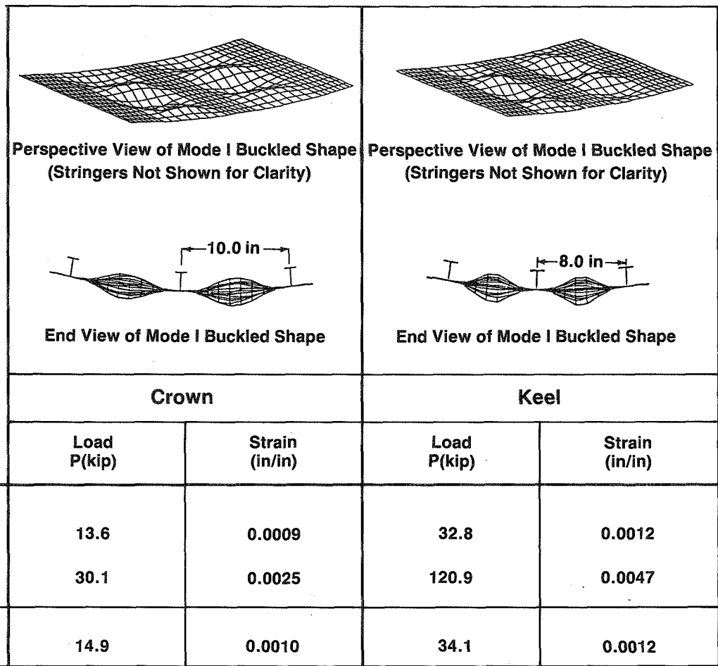
Figure 128. Nineteen-Shell STAGSC Buckling Analysis of Skin-Stringer Crown and Keel (Test 4)
