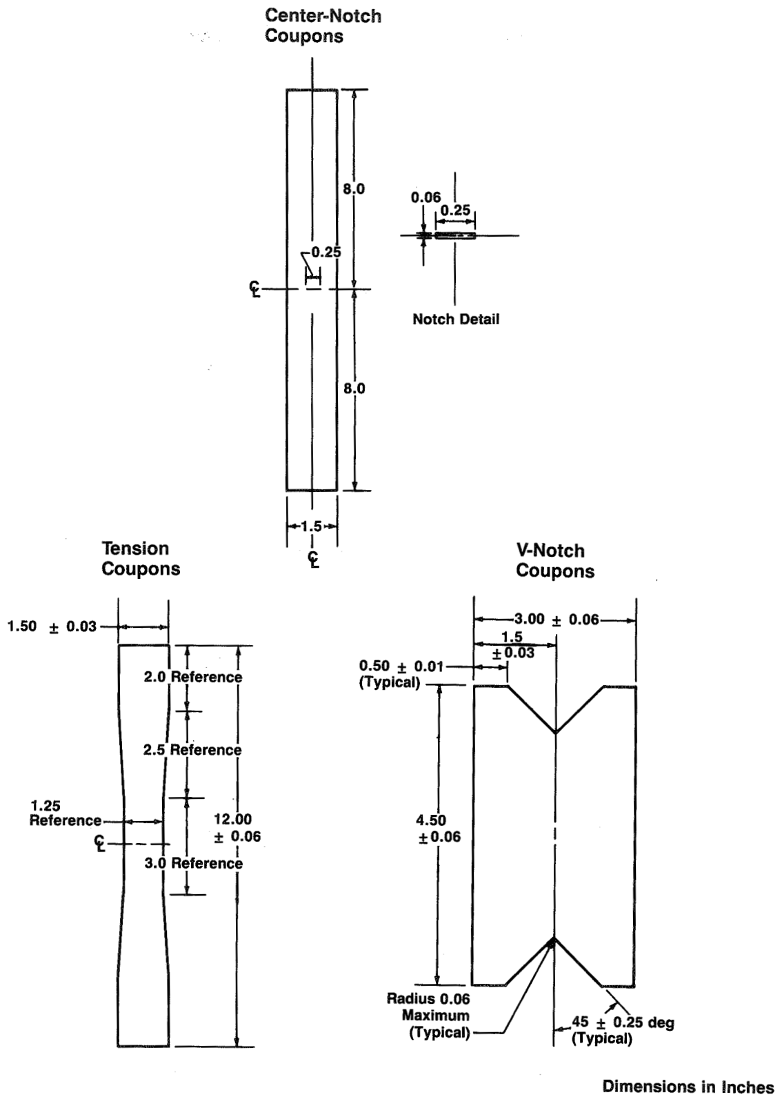
Figure 94. Coupon Specimens To Determine Panel Properties for Use in Model Analysis
