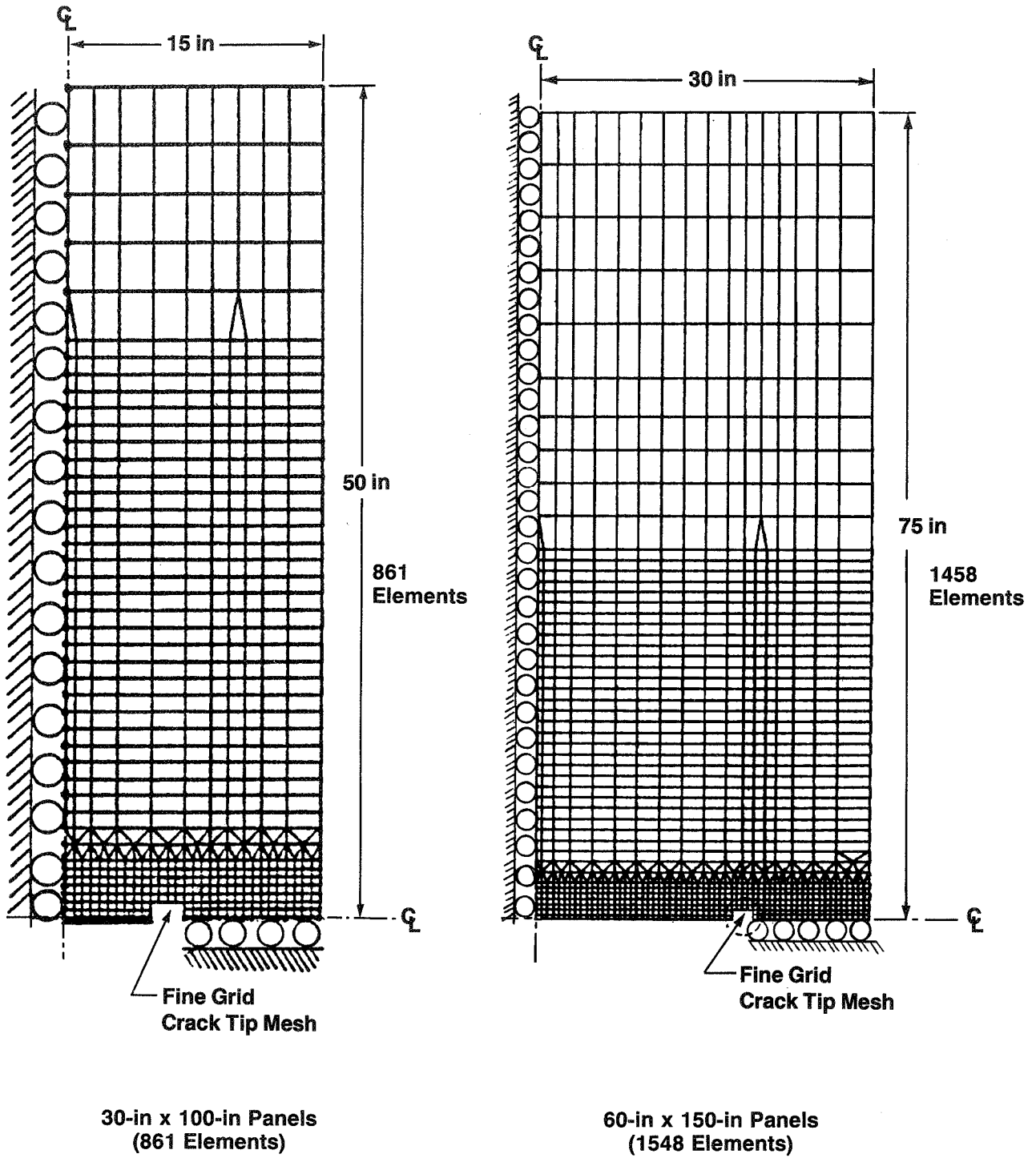
Figure 86. Finite Element Models for Flat Fracture Panel Tests
