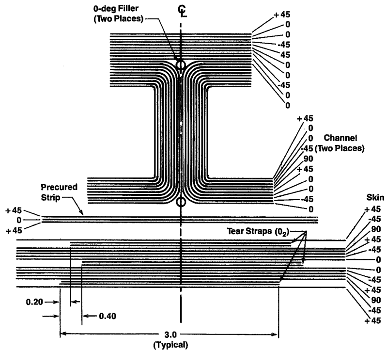
b. Keel Station 1200
