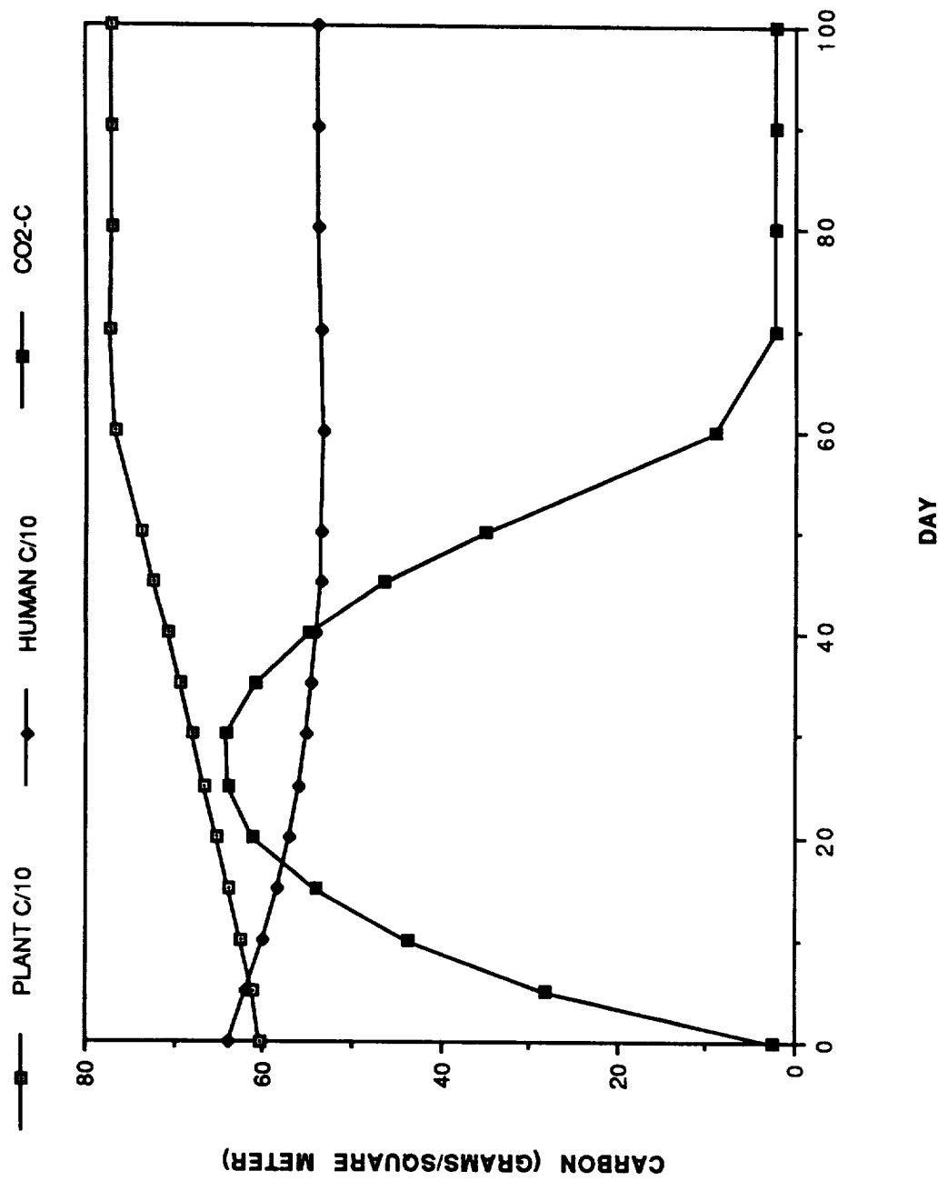
Figure 6. Effects of decreasing initial plant biomass by a third in CELSS model with Michaelis-Menten kinetics describing photosynthesis.
