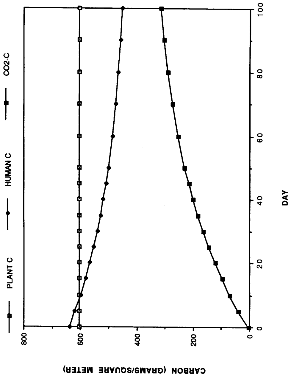
Figure 5. Effects of decreasing initial plant biomass by a third in CELSS model with recipient control photosynthetic flux.
