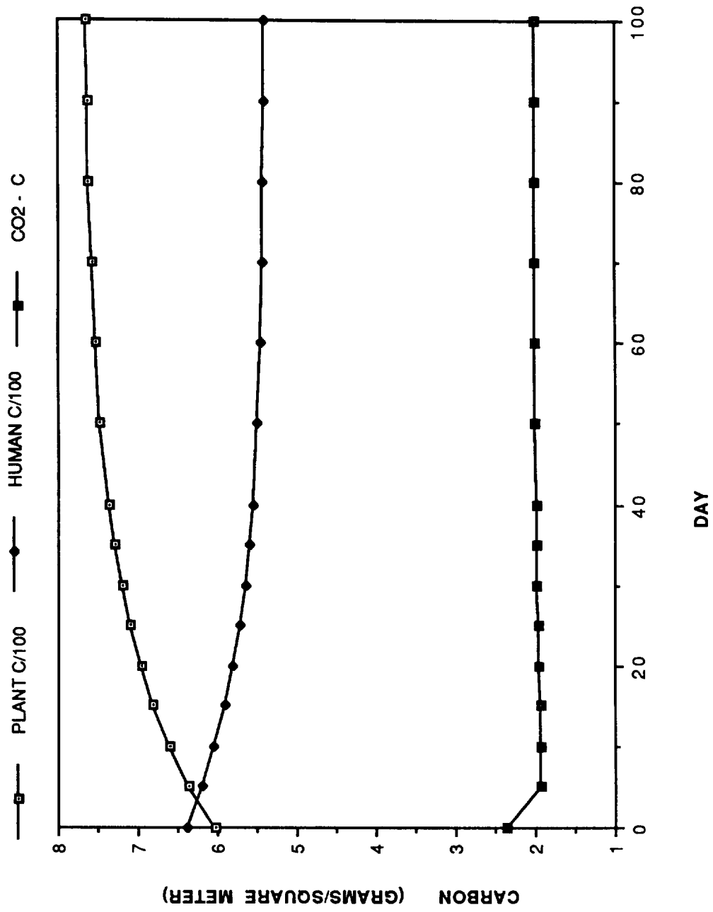
Figure 4. Effects of decreasing initial plant biomass by a third in CELSS model with donor-controlled photosynthetic flux.
