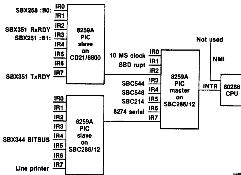
Fig. 10 Central system interrupt configuration.
