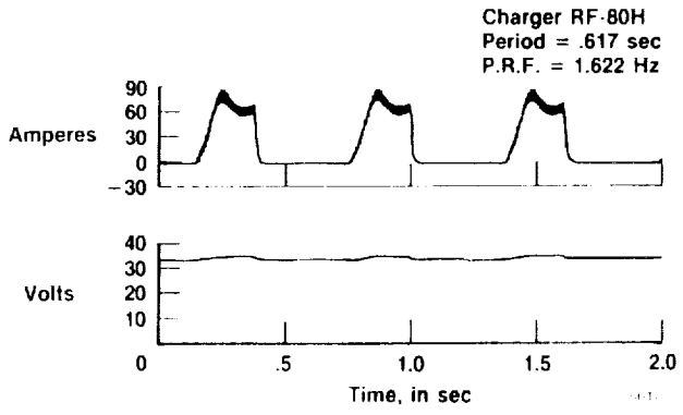
Fig. 19 Reflex charging waveforms.
