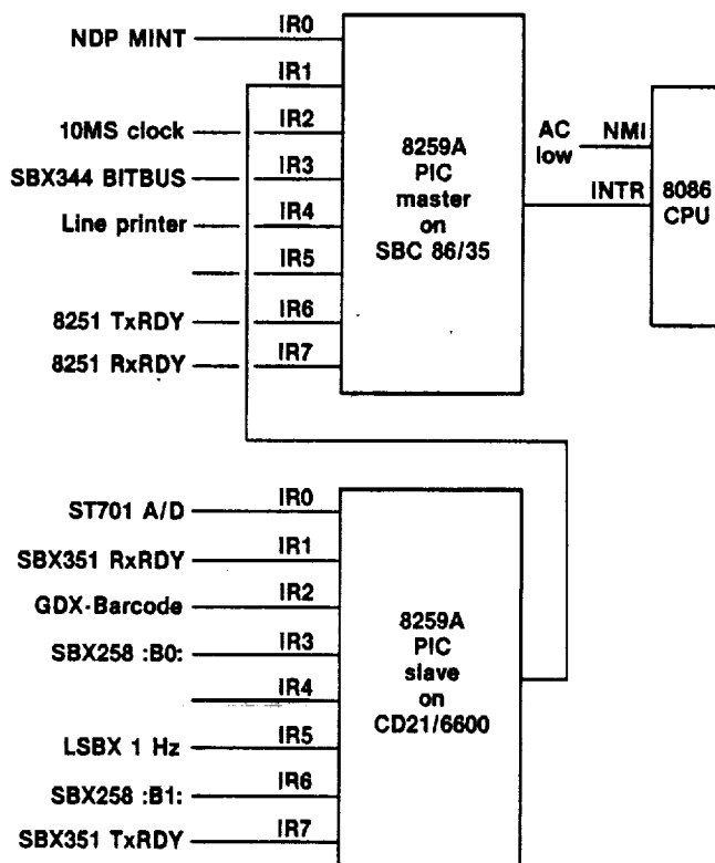
Fig. 14 BSC interrupt configuration.
