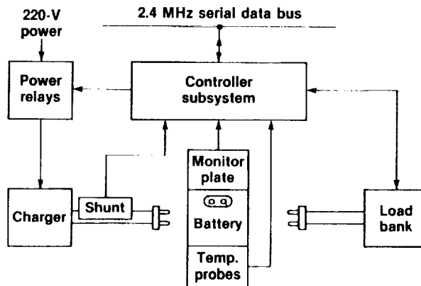
Fig. 3 AESL battery station overview.
