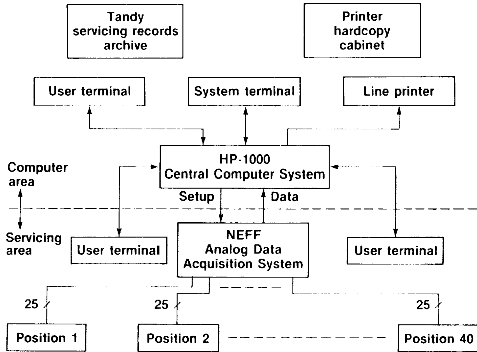
Fig. 1 Battery Systems Laboratory overview.
