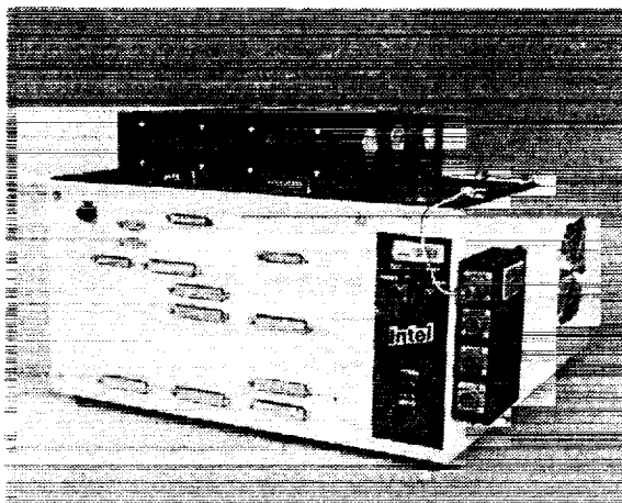
Fig. 11 Battery station controller subsystem chassis.
