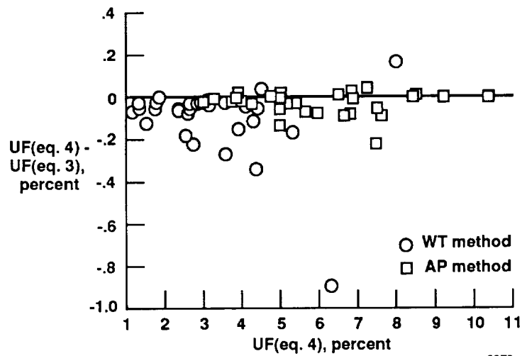
Fig. 6 Nonlinearity effects on equation (4) thrust uncertainty results.
