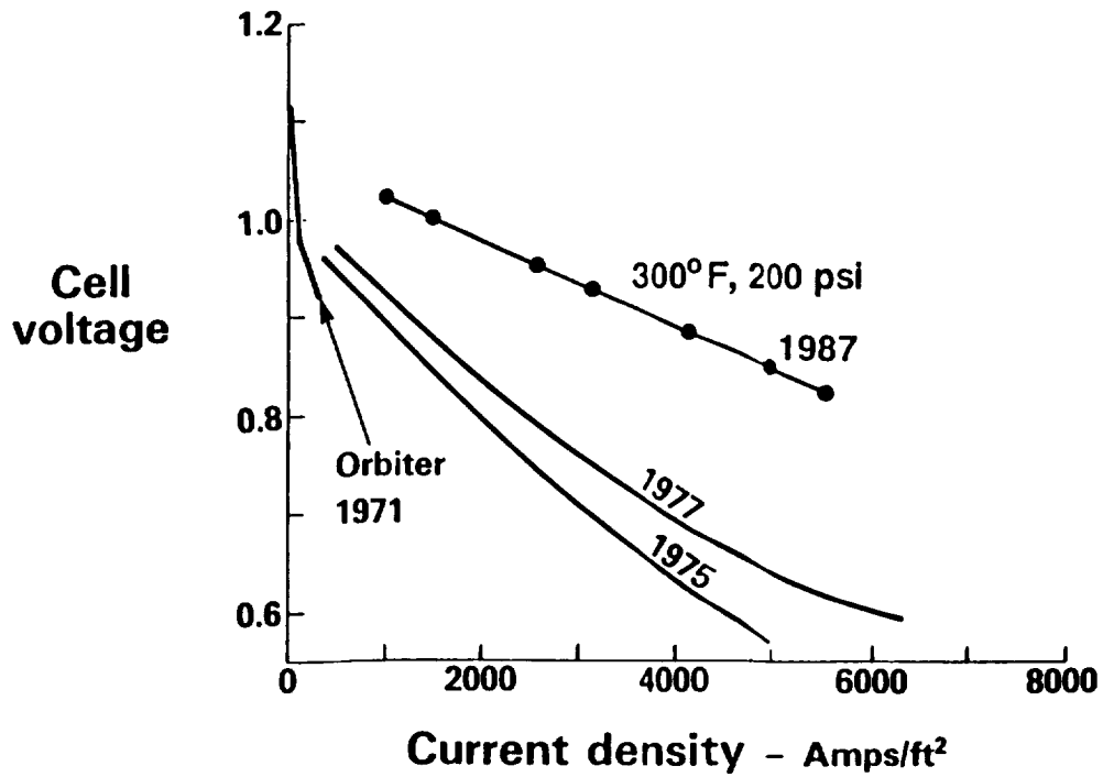
FIGURE 3: ALKALINE HIGH POWER DENSITY PERFORMANCE
