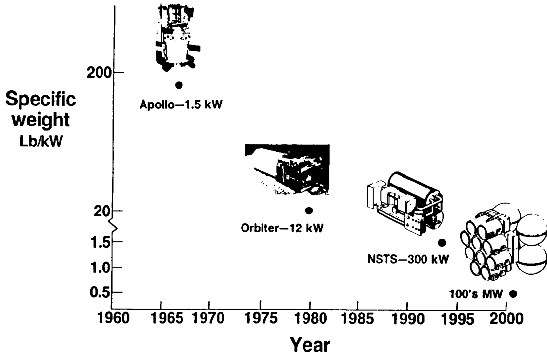
FIGURE 4: PROGRESS IN FUEL CELL SPACE POWER
