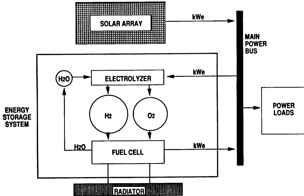
FIGURE 1: REGENERATIVE FUEL CELL SYSTEM SCHEMATIC
