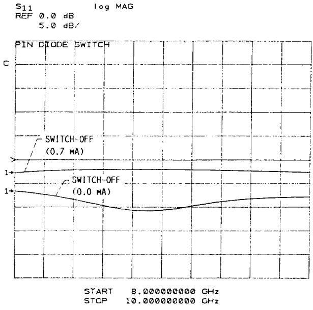
(b) MEASURED RETURN LOSS.
