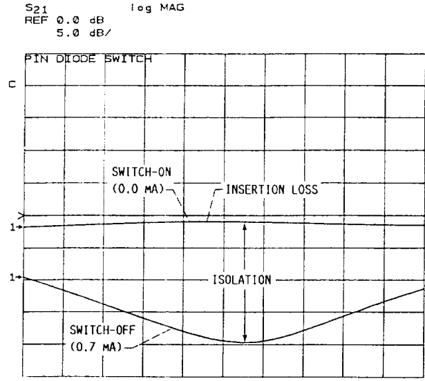
(a) MEASURED INSERTION LOSS AND ISOLATION.
