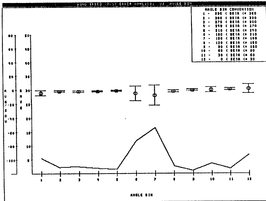
Fig. 7 Errors in total wind speed estimates from a simulated space-based lidar scan.
