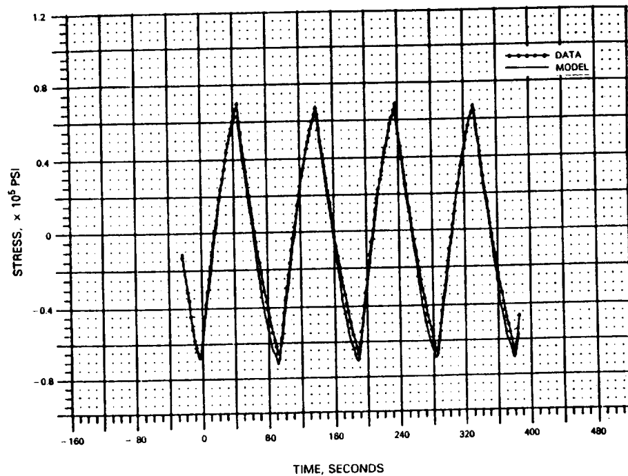
FIGURE 4.16. FIT OF 1600°F, FULLY REVERSED, RAPID CYCLE DATA AT +.4% (SPECIMEN 31B) USING WALKER'S MODEL WITH CONSTANTS DERIVED FROM SPECIMEN 27B.
