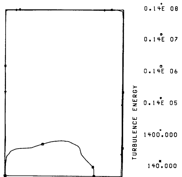
FIGURE 41. - NATURAL LOGARITHM OF TURBULENT KINETIC ENERGY PROFILES AT 350° ATDC FOR 22.5° SWIRL ANGLE.
