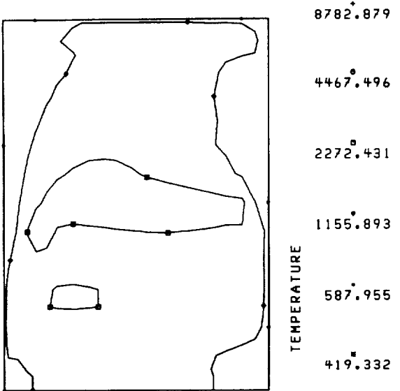
FIGURE 34. - TEMPERATURE ISOCONTOURS AT 40° ATDC FOR 22.5° SWIRL ANGLE.
