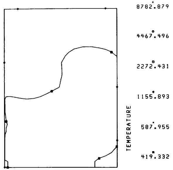
FIGURE 9. - TEMPERATURE ISOCONTOURS AT 356° ATDC FOR 22.5° SWIRL ANGLE.
