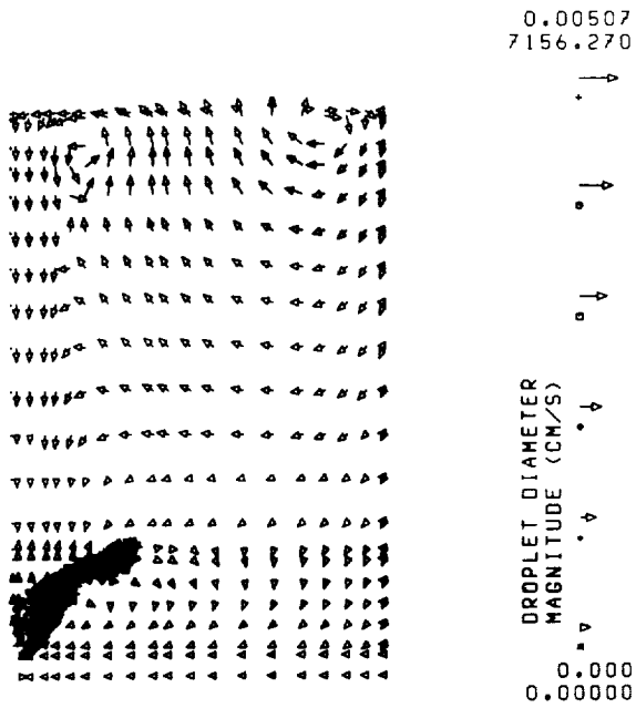
FIGURE 2. - GAS PHASE VELOCITY VECTOR PROFILES AND DROPLET LOCATIONS AT 350 0 ATDC FOR 22.5 0 SWIRL ANGLE.
