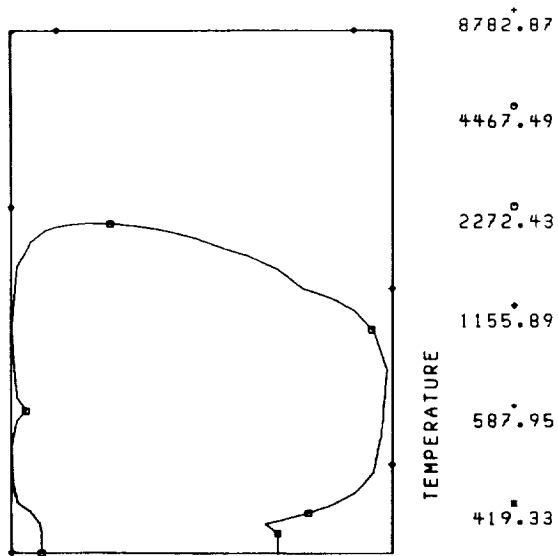
FIGURE 24. - TEMPERATURE ISOCONTOURS AT 5 0 ATDC FOR 22.5 0 SWIRL ANGLE.
