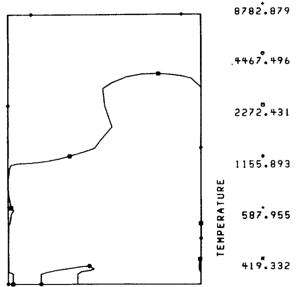
FIGURE 11. - TEMPERATURE ISOCONTOURS AT 357° ATDC FOR 22.5° SWIRL ANGLE.
