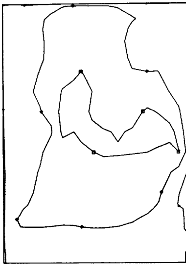
FIGURE 38. - TEMPERATURE ISOCONTOURS AT 80° ATDC FOR 22.5° SWIRL ANGLE.
