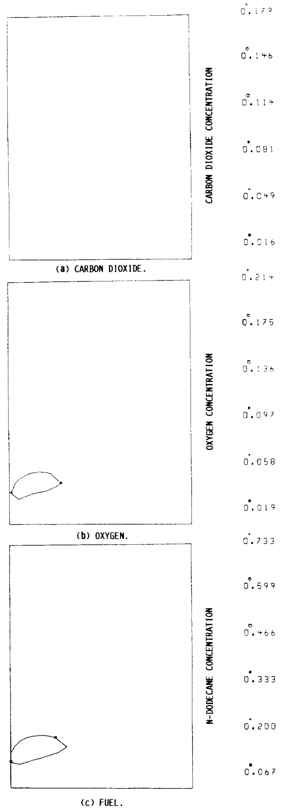
FIGURE 3. - MASS FRACTION DISTRIBUTIONS AT 350 0 ATDC FOR
