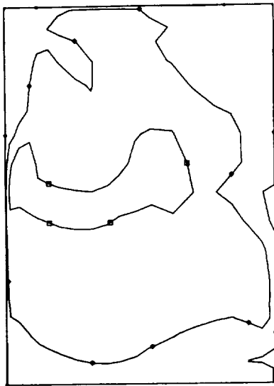
FIGURE 36. - TEMPERATURE ISOCONTOURS AT 60° ATDC FOR 22.5° SWIRL ANGLE.
