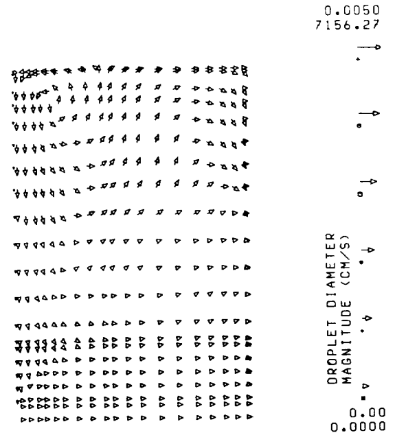
FIGURE 31. - GAS PHASE VELOCITY VECTOR PROFILES AND DROPLET LOCATIONS AT 30 0 ATDC FOR 22.5 0 SWIRL ANGLE.
