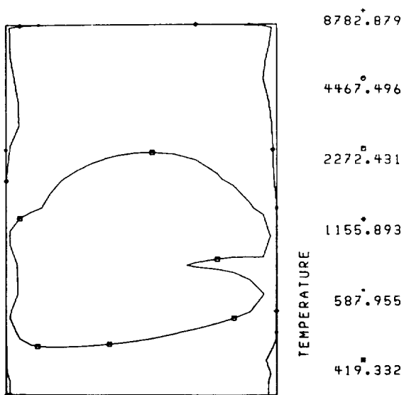
FIGURE 30. - TEMPERATURE ISOCONTOURS AT 20 0 ATDC FOR 22.5 0 SWIRL ANGLE.
