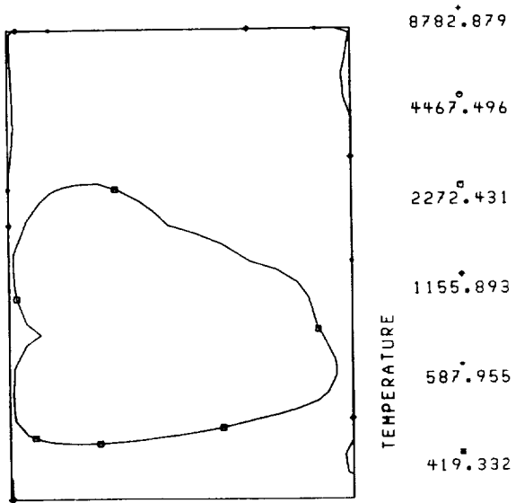
FIGURE 28. - TEMPERATURE ISOCONTOURS AT 15 0 ATDC FOR 22.5 0 SWIRL ANGLE.
