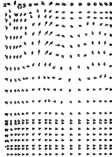
FIGURE 37. - GAS PHASE VELOCITY VECTOR PROFILES AT 80° ATDC FOR 22.5° SWIRL ANGLE.
