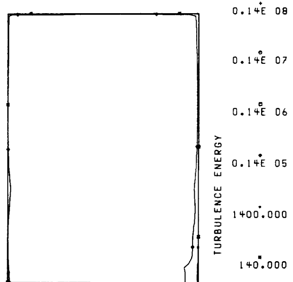
FIGURE 43. - NATURAL LOGARITHM OF TURBULENT KINETIC ENERGY PROFILES AT 10° ATDC FOR 22.5° SWIRL ANGLE.
