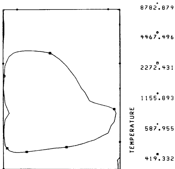
FIGURE 26. - TEMPERATURE ISOCONTOURS AT 10 0 ATDC FOR 22.5 0 SWIRL ANGLE.
