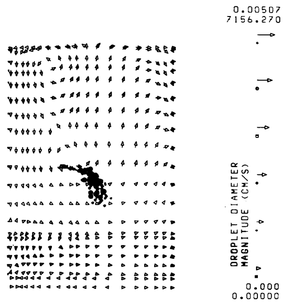
FIGURE 29. - GAS PHASE VELOCITY VECTOR PROFILES AND DROPLET LOCATIONS AT 20 0 ATDC FOR 22.5 0 SWIRL ANGLE.
