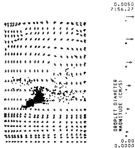
FIGURE 25. - GAS PHASE VELOCITY VECTOR PROFILES AND DROP-LET LOCATIONS AT 10 0 ATDC FOR 22.5 0 SWIRL ANGLE.
