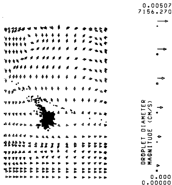
FIGURE 27. - GAS PHASE VELOCITY VECTOR PROFILES AND DROP-LET LOCATIONS AT 15 0 ATDC FOR 22.5 0 SWIRL ANGLE.
