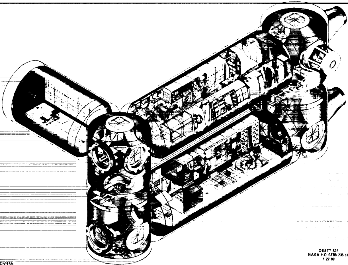
FIGURE 2. - U.S. LABORATORY, HABITATION, AND LOGISTICS MODULES AND CONNECTING NODES.
