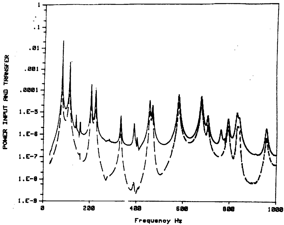
Figure 7. Power input and transfer per unit acoustic pressure with the influence of fluid loading for angle of incidence \phi and \theta equal 0^\circ and 90^\circ respectively. —: Power input; ---: power transfer.
