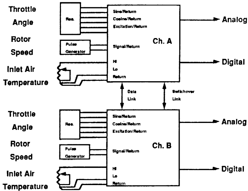
Figure 5: Simulated EEC Inputs for TRA, N1, T2
