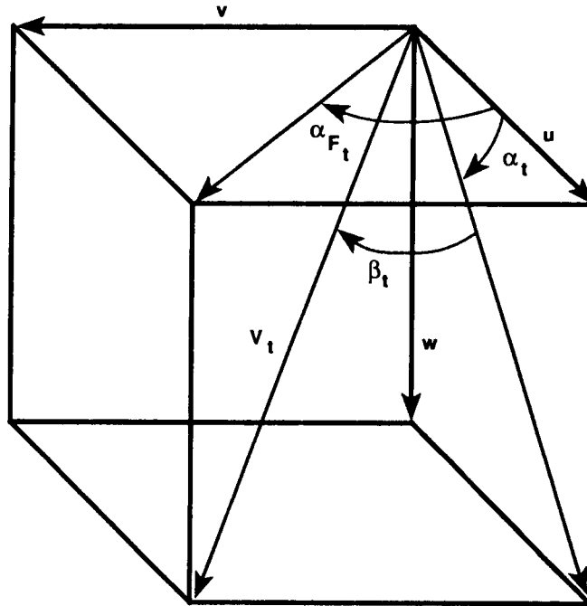
Fig. 9 Flow angle definitions.
