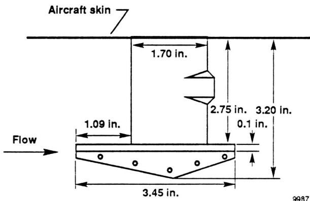
Fig. 3 Nondeiced, open element, total temperature sensor.
