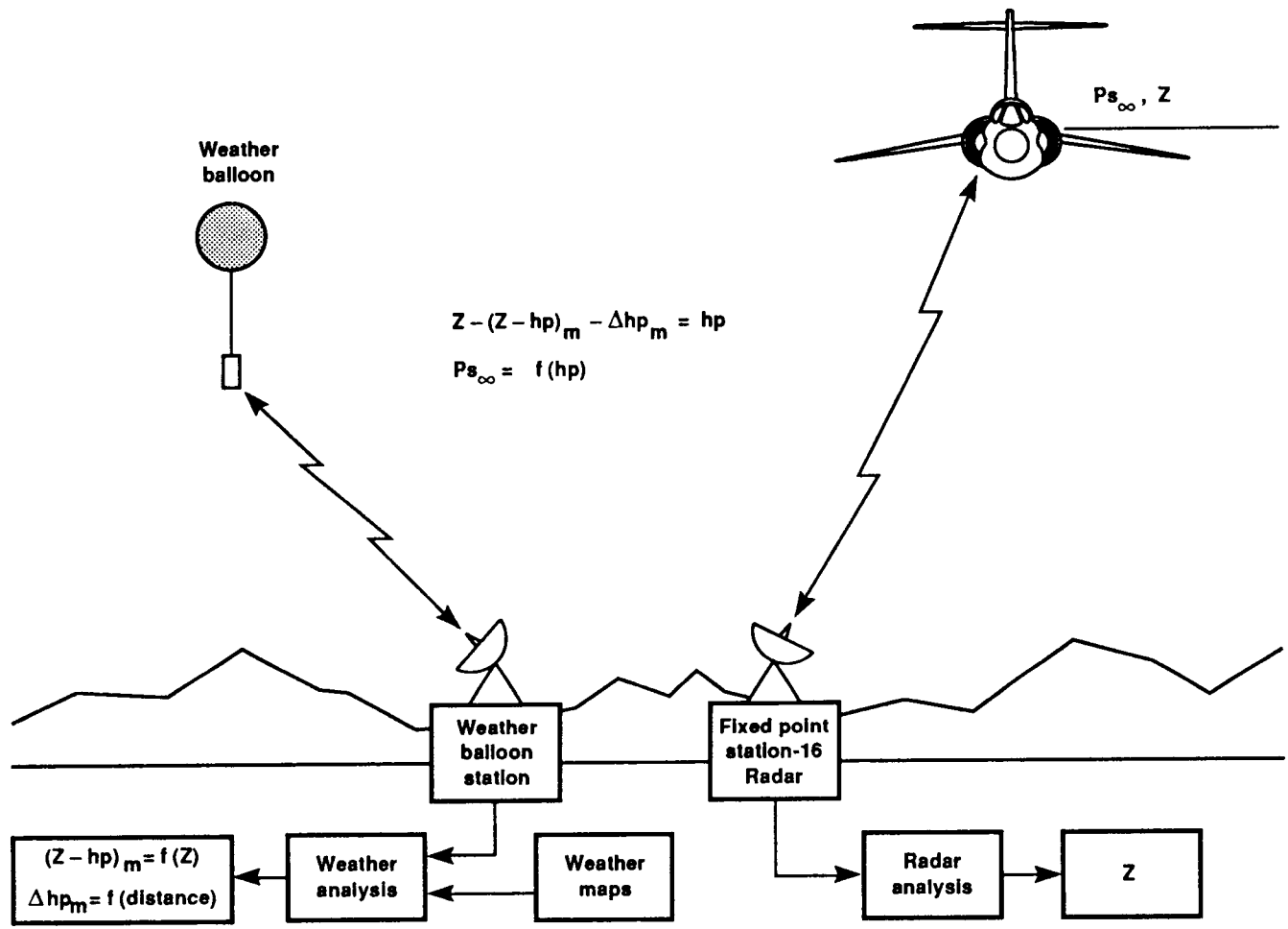
Fig. 6 Radar acceleration-deceleration position error calibration method.
