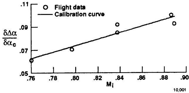
Fig. 15 Subsonic upwash factor.
