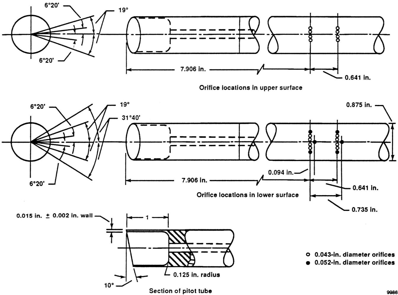
(b) Total and static port configurations.
