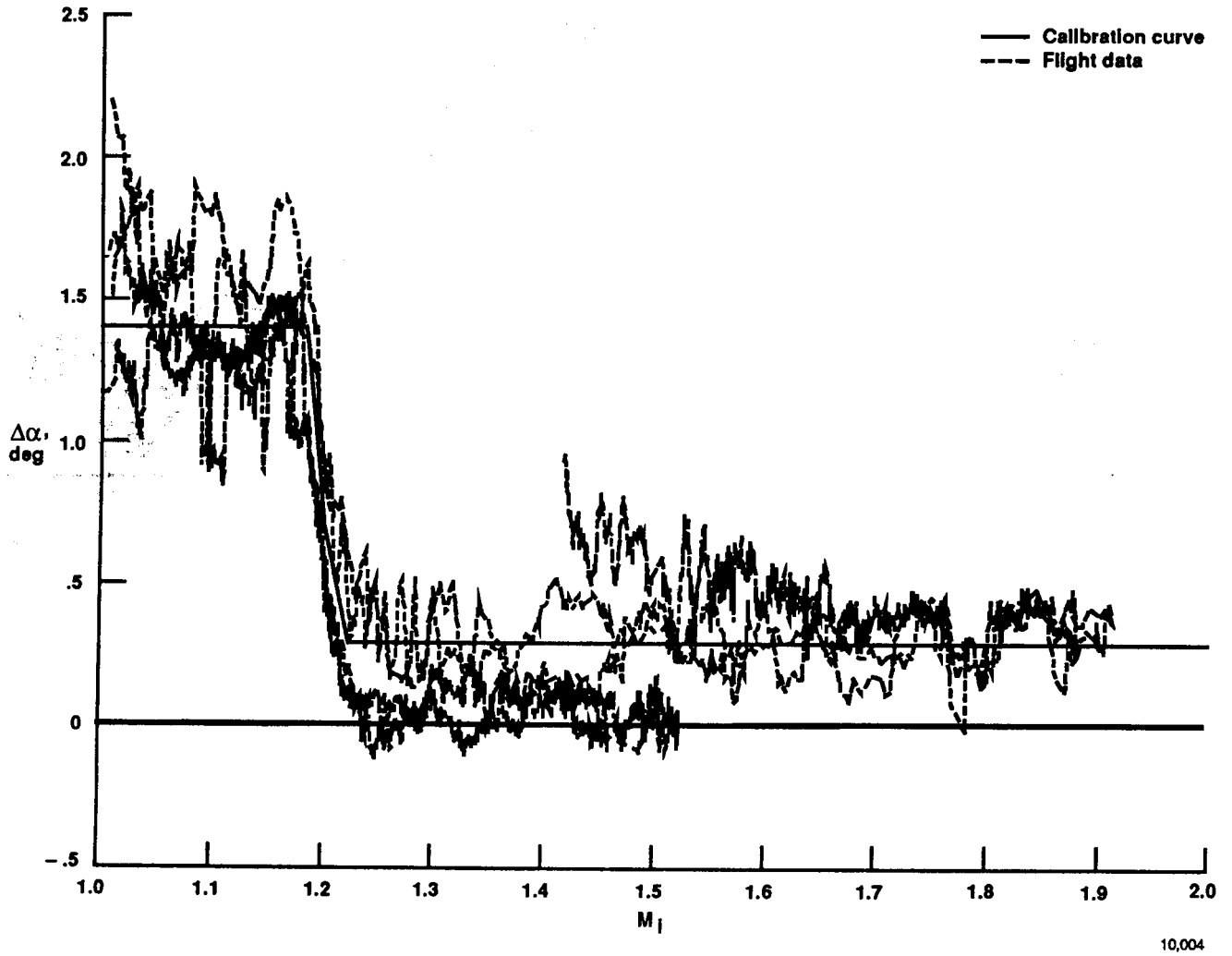
Fig. 18 Supersonic angle-of-attack calibration.
