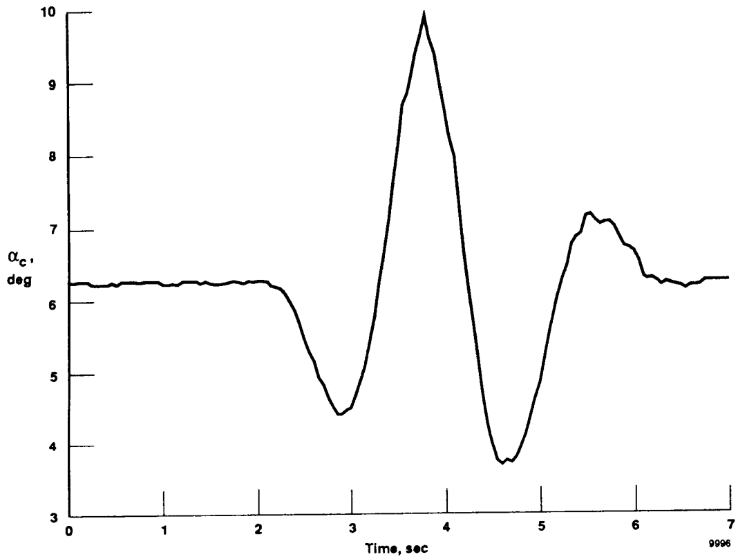
(a) Angle of attack.
