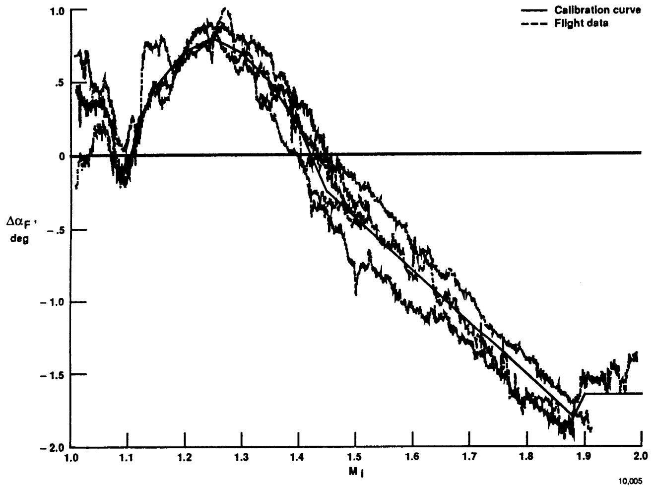
Fig. 19 Supersonic angle-of-sideslip calibration.
