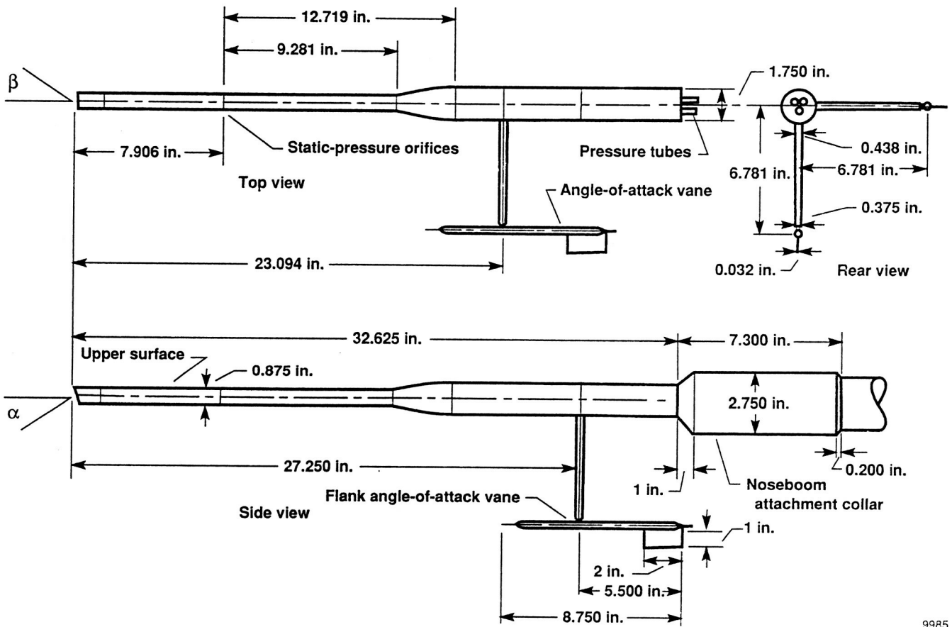
(a) Airdata probe with noseboom attachment collar.
