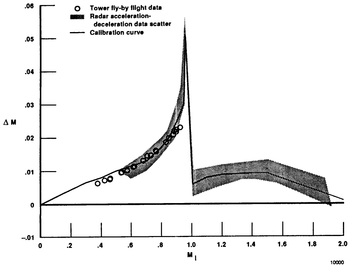
Fig. 14 Mach number position error calibration.
