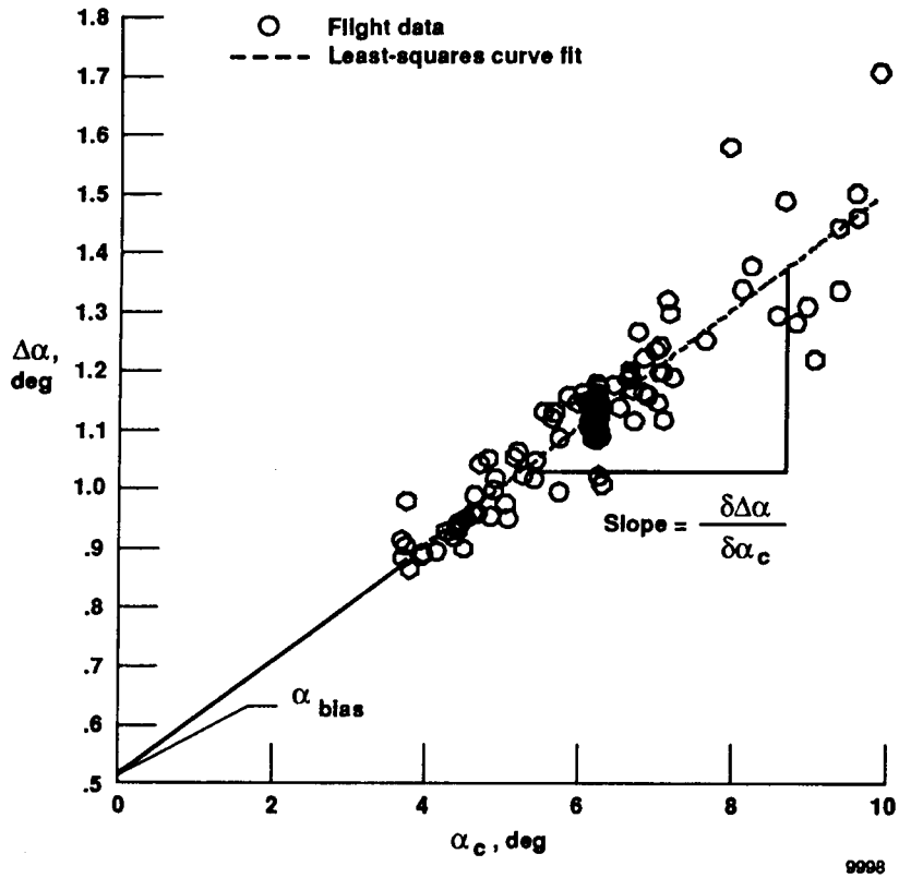
(a) Angle of attack.
