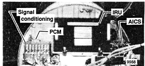
Fig. 4 The IRU, AICS, PCM system, and signal conditioning installed in aircraft.
