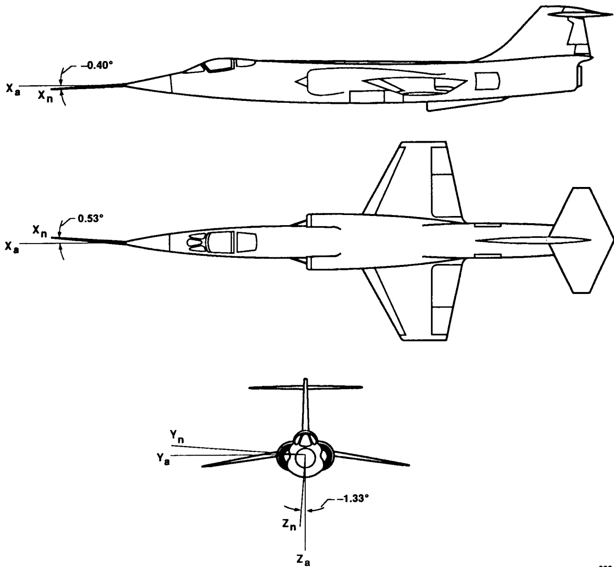
Fig. 10 Noseboom offset angles for check 1.
