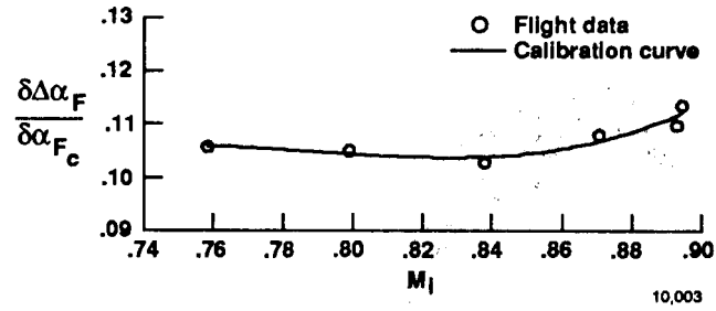
Fig. 17 Subsonic sidewash factor.
