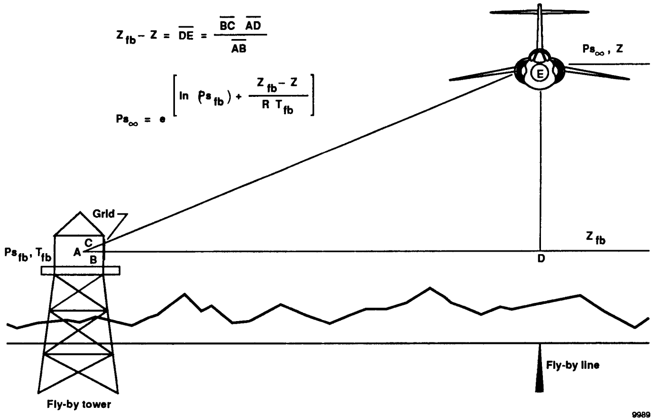
Fig. 5 Tower fly-by position error calibration method.
