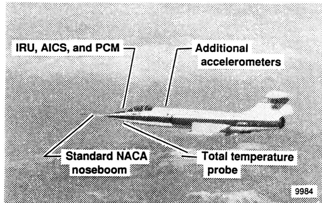
Fig. 1 The F-104 aircraft.
