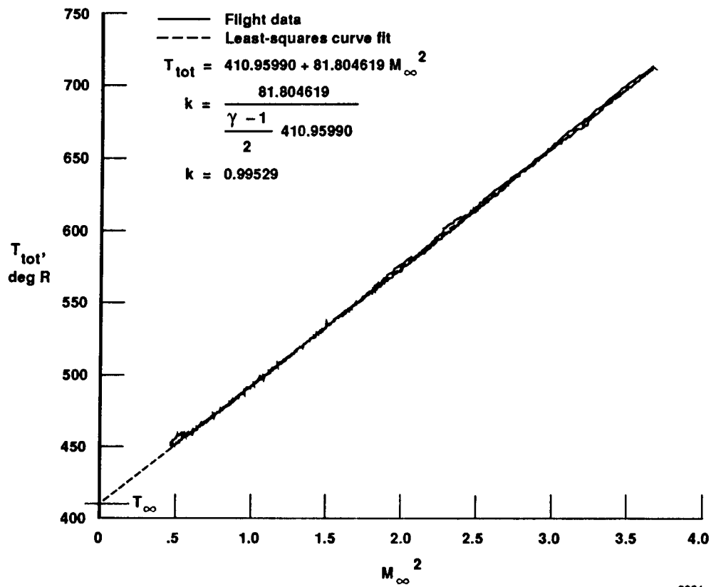
Fig. 7 Total temperature recovery factor calibration technique.
