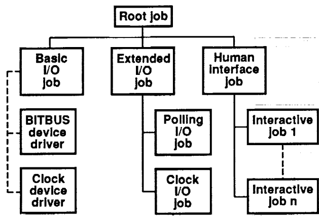
Figure 10. Central system software.
