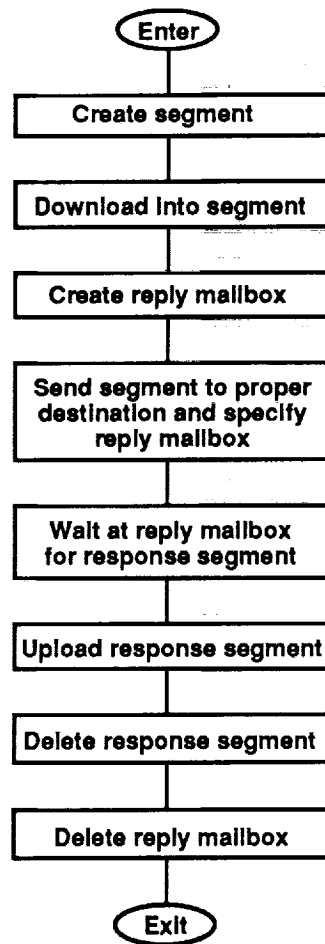
Figure 7. iRMX object based protocol.
