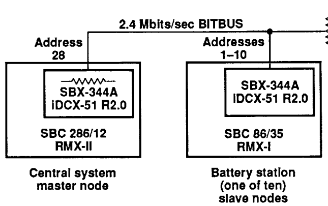
Figure 4. BITBUS hardware configuration.
