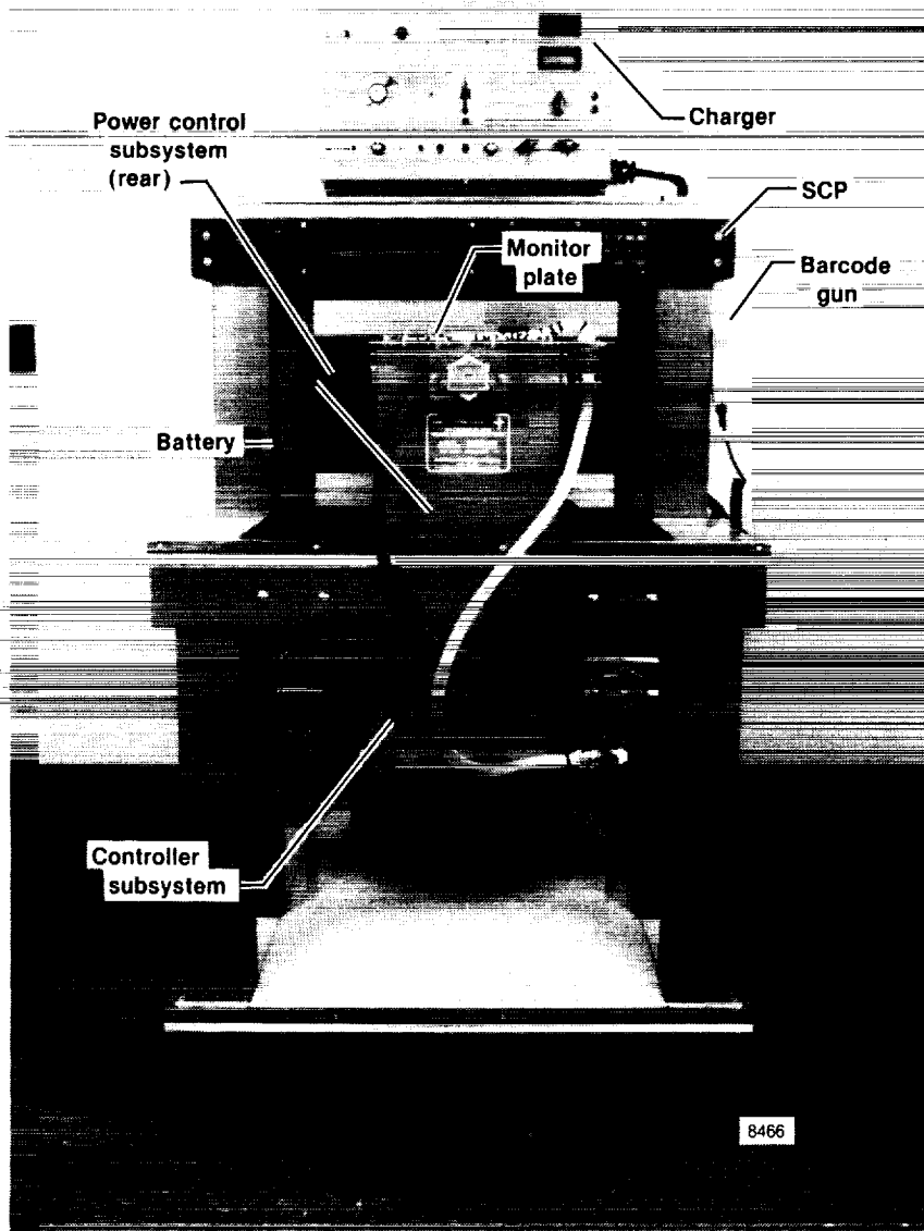
Figure 2. Battery station bench.
