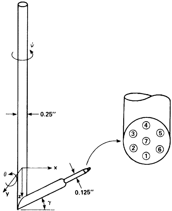
Figure 6.— Seven hole probe and hole numbering convention.
