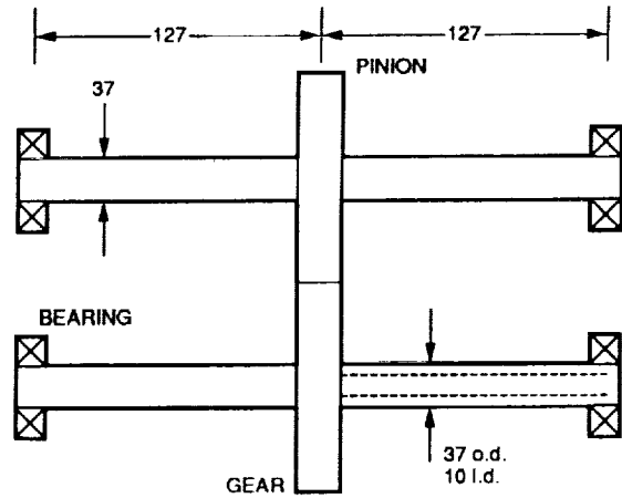
Figure 6. - The system analyzed as a third example. (Dimensions are in millimeters.)
