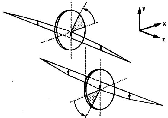
(b) Natural frequency, 2524 Hz.
