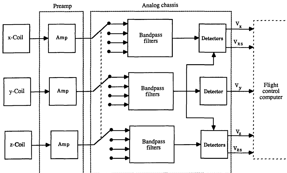
Figure 6. Simplified block diagram of aircraft subsystem.
