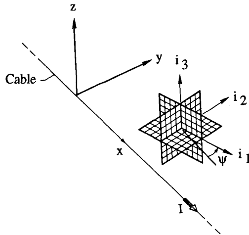
Figure 3. Coil geometry.
