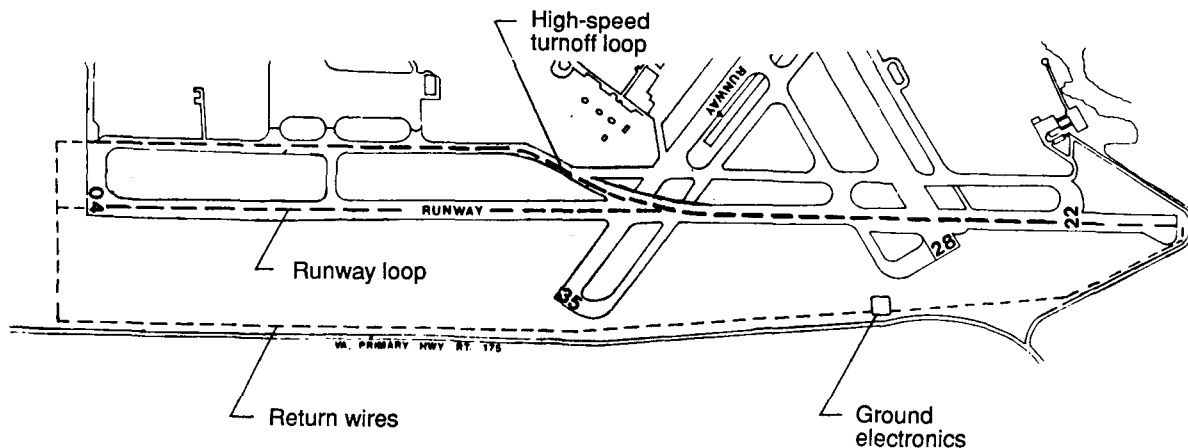
Figure 4. MLC installation at Wallops Flight Facility.
