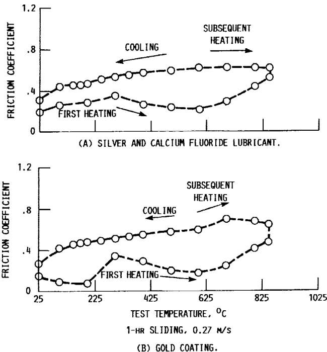
FIGURE 23. - FRICTION COEFFICIENT FOR FABRIC SLIDING AGAINST INCONEL TEST DISK.
