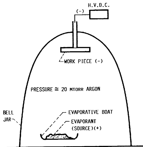
FIGURE 20. - ION PLATING.
