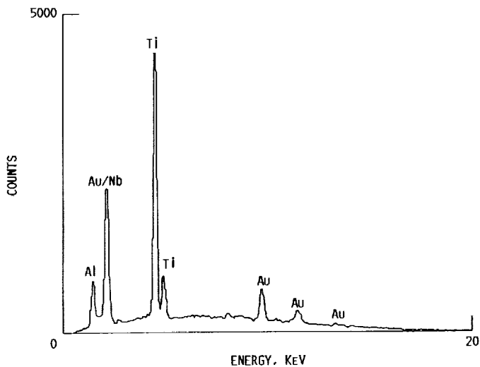
FIGURE 33. - EDS X-RAY SPECTRUM OF Ti 3 Al-Nb DISK ION PLATED WITH GOLD AFTER SLIDING AGAINST FABRIC AT 700 °C. SURFACE SCRAPED PRIOR TO ANALYSIS.
