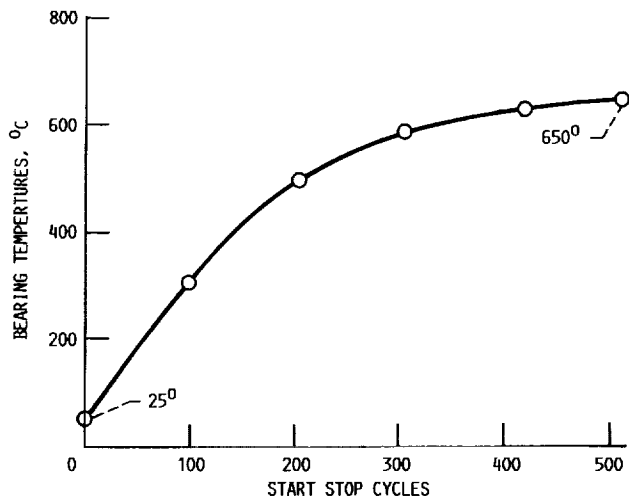
FIGURE 6. - TEST TEMPERATURE DURING 500 START/STOP CYCLES HEATING FROM 25 °C TO 650 °C.
