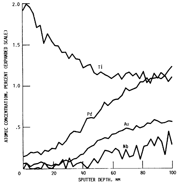
FIGURE 29. - XPS DEPTH PROFILE RESULTS OF HEAT TREATED INTER-METALLIC WHICH WAS COATED WITH 50 NM PALADIUM AND 100 NM OF GOLD.
