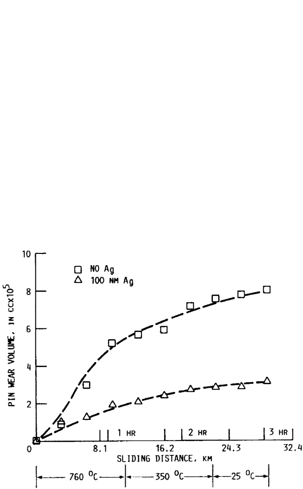
FIGURE 14. - PIN WEAR VOLUME VERSUS SLIDING DISTANCE. TEST CONDITIONS: 4.9 N LOAD, 2.7 m/s SLIDING VELOCITY, HELIUM ATMOSPHERE.
