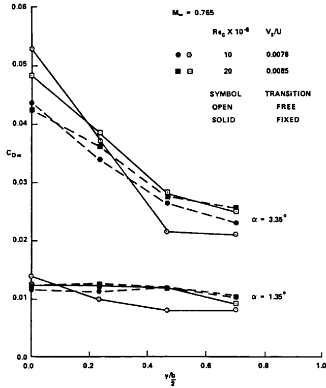
SPANWISE WAKE DRAG VARIATION AT VARIOUS REYNOLDS NUMBERS FOR TWO ANGLES OF ATTACK WITH FIXED OR FREE TRANSITION, M_\infty = 0.765
