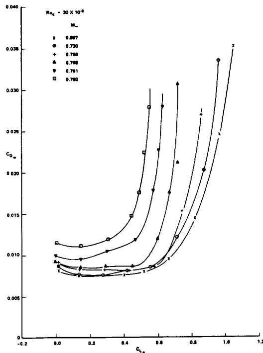
DRAG VERSUS LIFT AT VARIOUS MACH NUMBERS AT NOMINAL Re_c = 30 \times 10^6 WITH FREE TRANSITION
