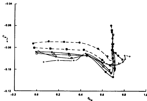
PITCHING MOMENT VERSUS LIFT AT VARIOUS REYNOLDS NUMBERS WITH FIXED OR FREE TRANSITION AT NOMINAL M_\infty = 0.765
