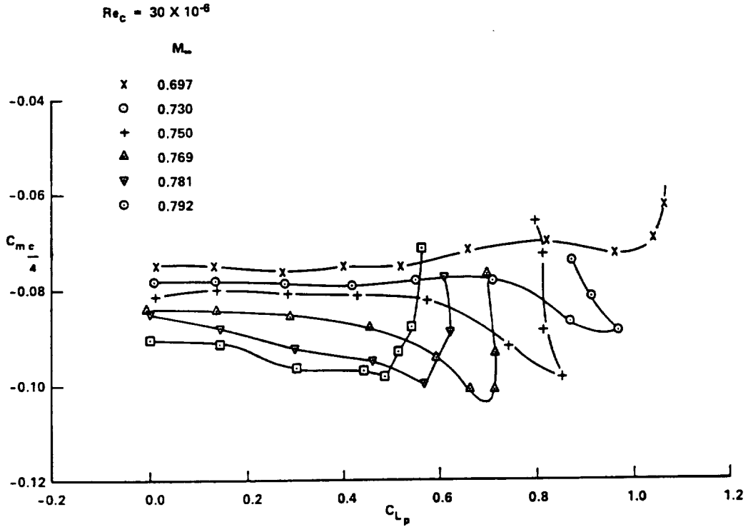
PITCHING MOMENT VERSUS LIFT AT VARIOUS MACH NUMBERS AT NOMINAL Re_c = 30 \times 10^6 WITH FREE TRANSITION
