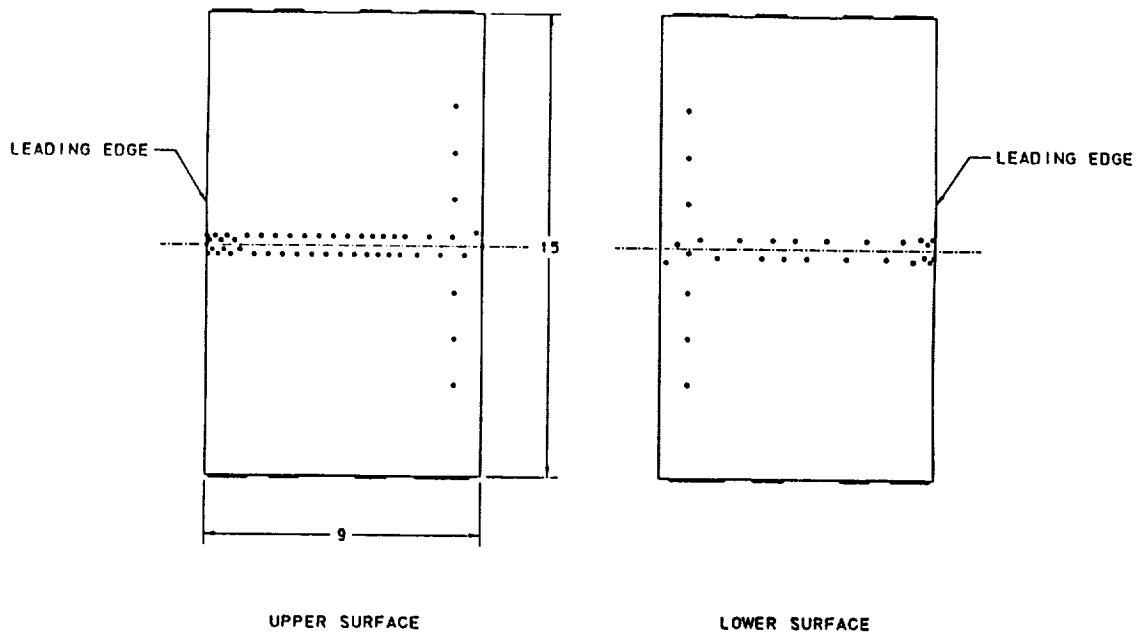
UPPER SURFACE LOWER SURFACE LOCATIONS OF PRESSURE ORIFICES AT UPPER AND LOWER SURFACES PLANE VIEW
