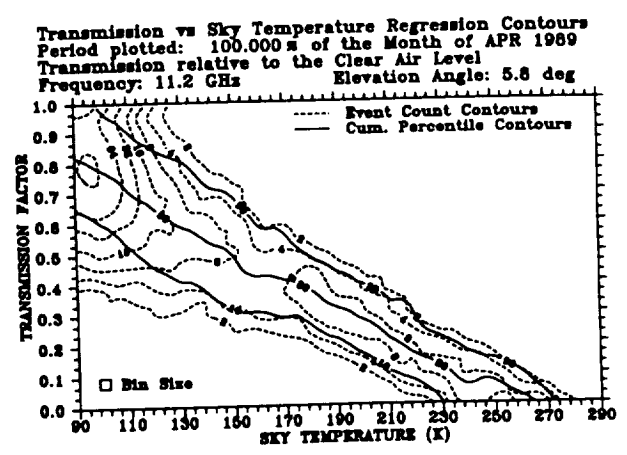
Fig. 6. Transmission factor vs. sky temperature regression contours
