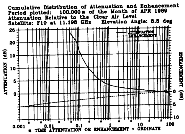
Fig. 3. Fade and enhancement distribution, Apr. 1989
