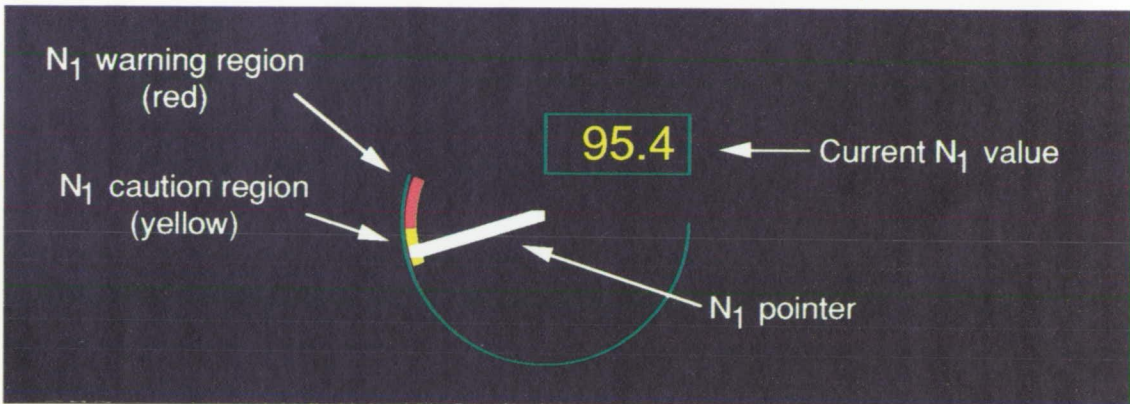
Figure 2. N 1 gauge.
