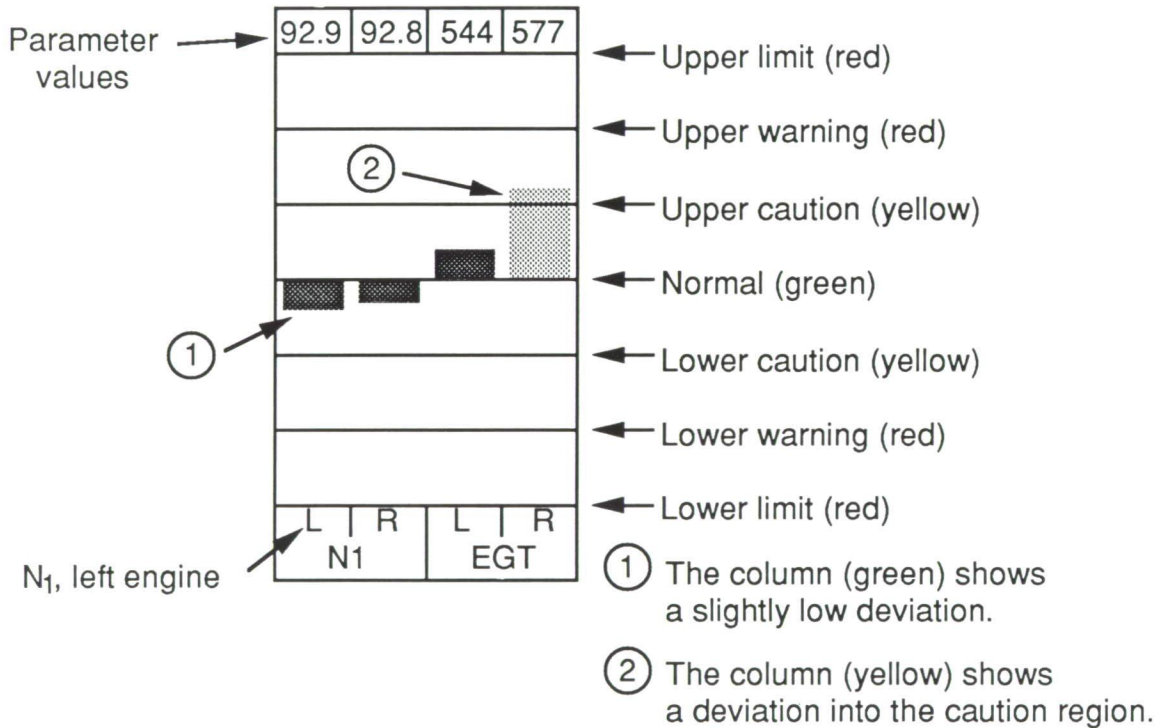
Figure A3. Representative monitoring indicators.
