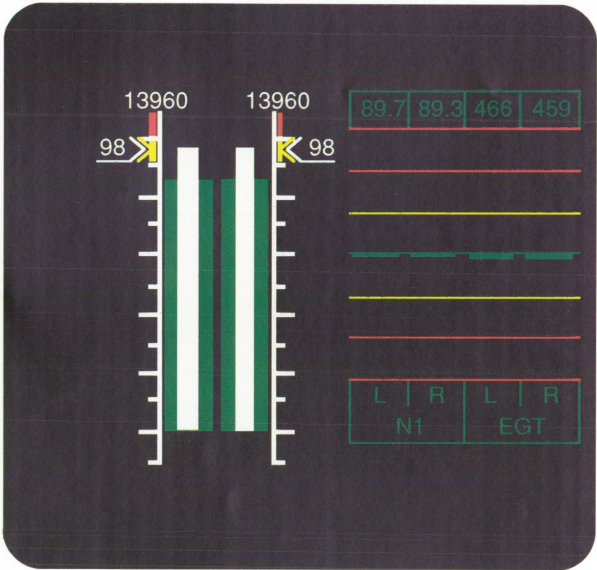
Figure 8. E-MACS display, left CRT.
