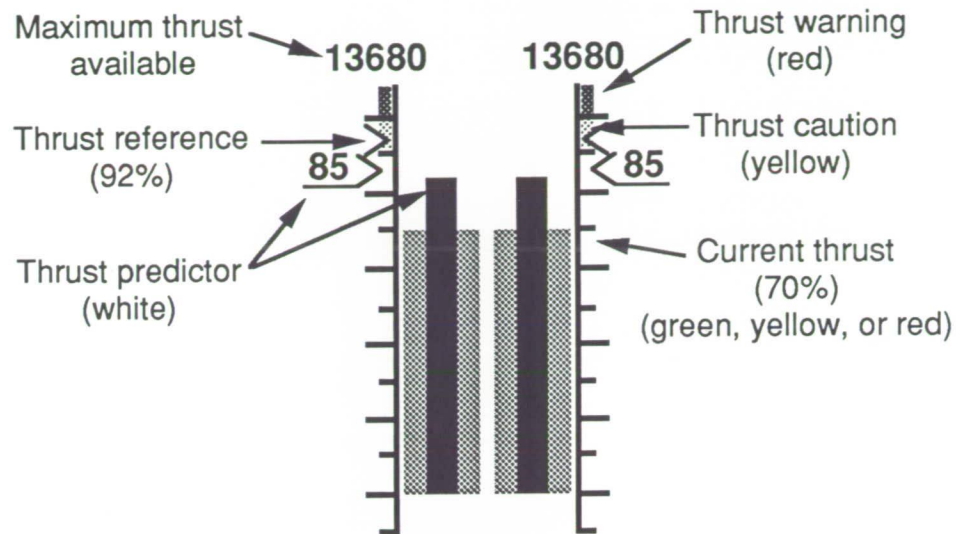
Figure A2. Thrust indicators.
