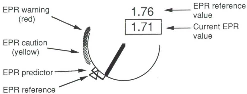
Figure A1. EPR gauge.
