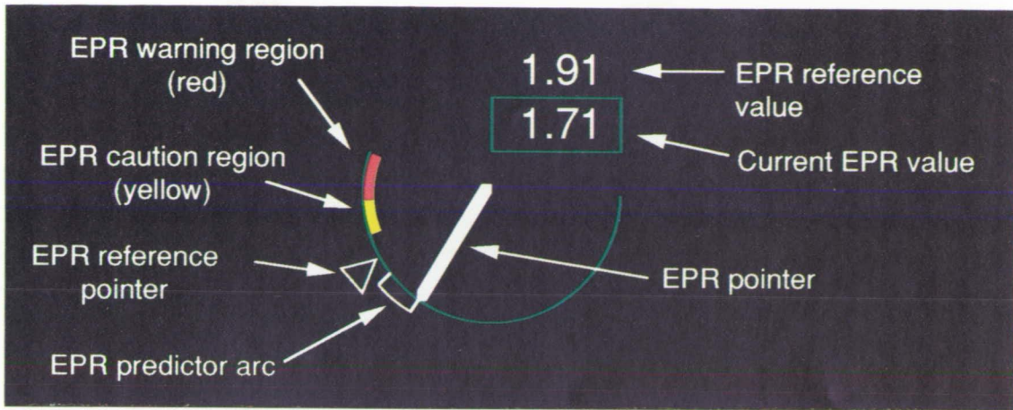
Figure 1. EPR gauge.
