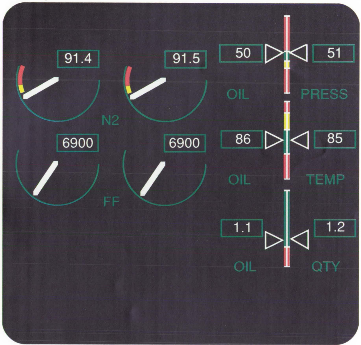
Figure 5. Traditional display, right CRT.
