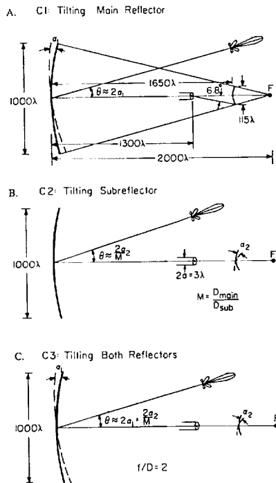
Figure 2. Cassegrain Dual Reflector Antenna Systems
